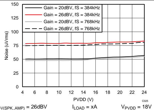
Figure 53. Idle Channel Noise vs PVDD – PBTL
