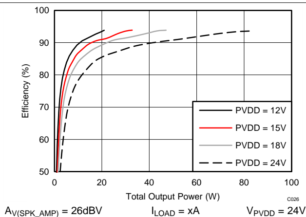
Figure 54. Efficiency vs Output Power – PBTL
