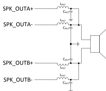
Figure 79. Post-Filter PBTB
