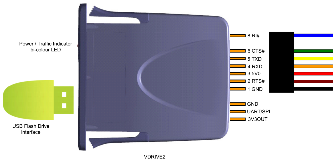
Figure 1 - VDrive2 Pin Out - UART interface.
