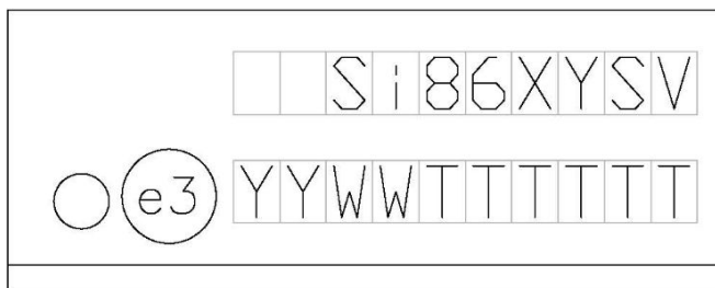
Figure 13.3. 16-Pin Narrow Body SOIC Top Marking
