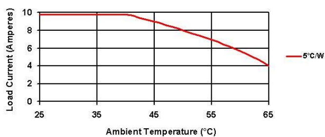
Derating Curve: DC200A10
