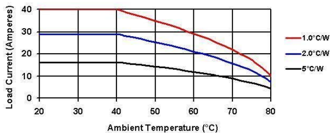
Derating Curve: DC200D20
