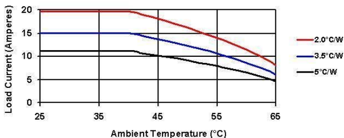
Derating Curve: DC200A20
