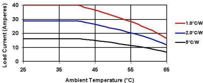
Derating Curve: DC200A20
