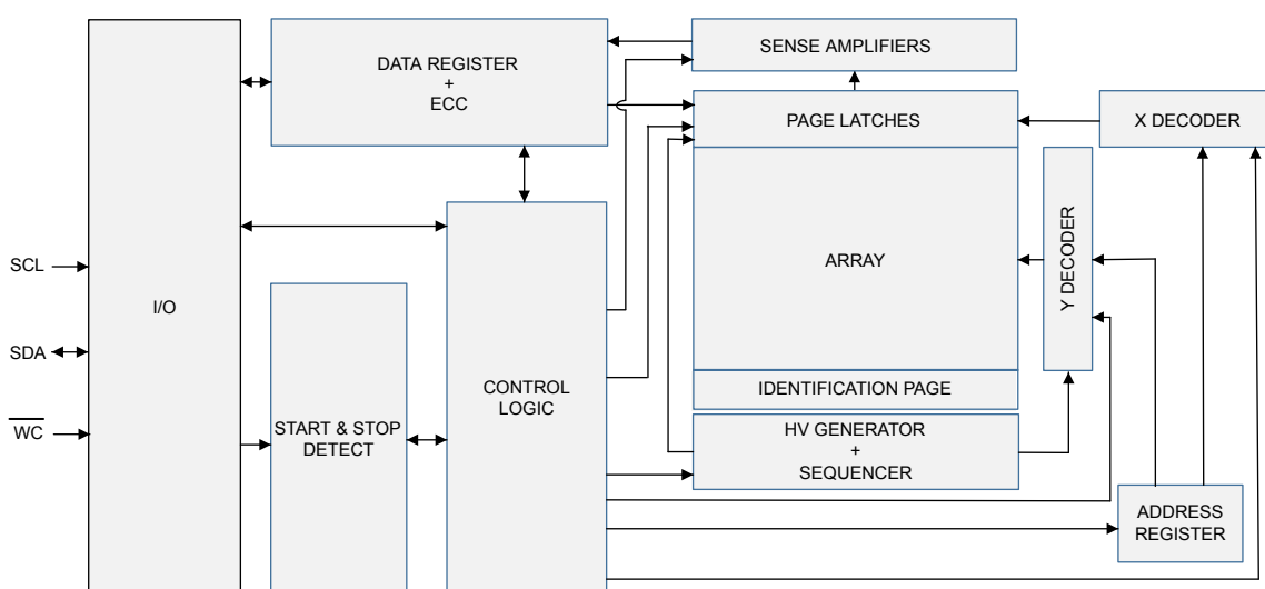
Figure 1. Logic diagram
