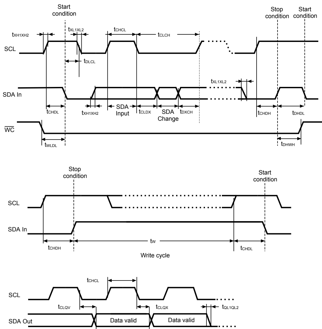
Figure 11. AC waveforms
