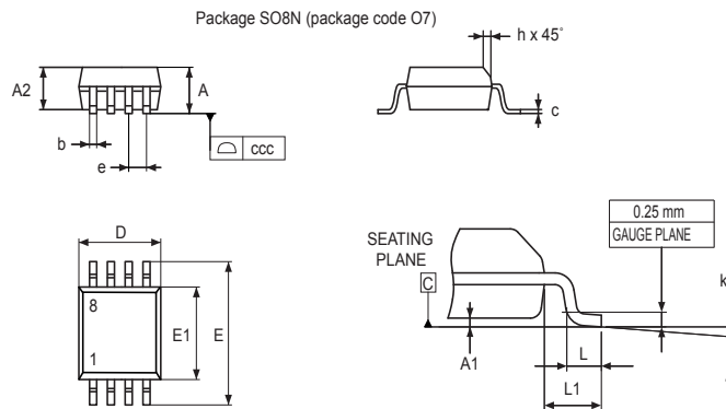
Figure 14. SO8N – Outline
