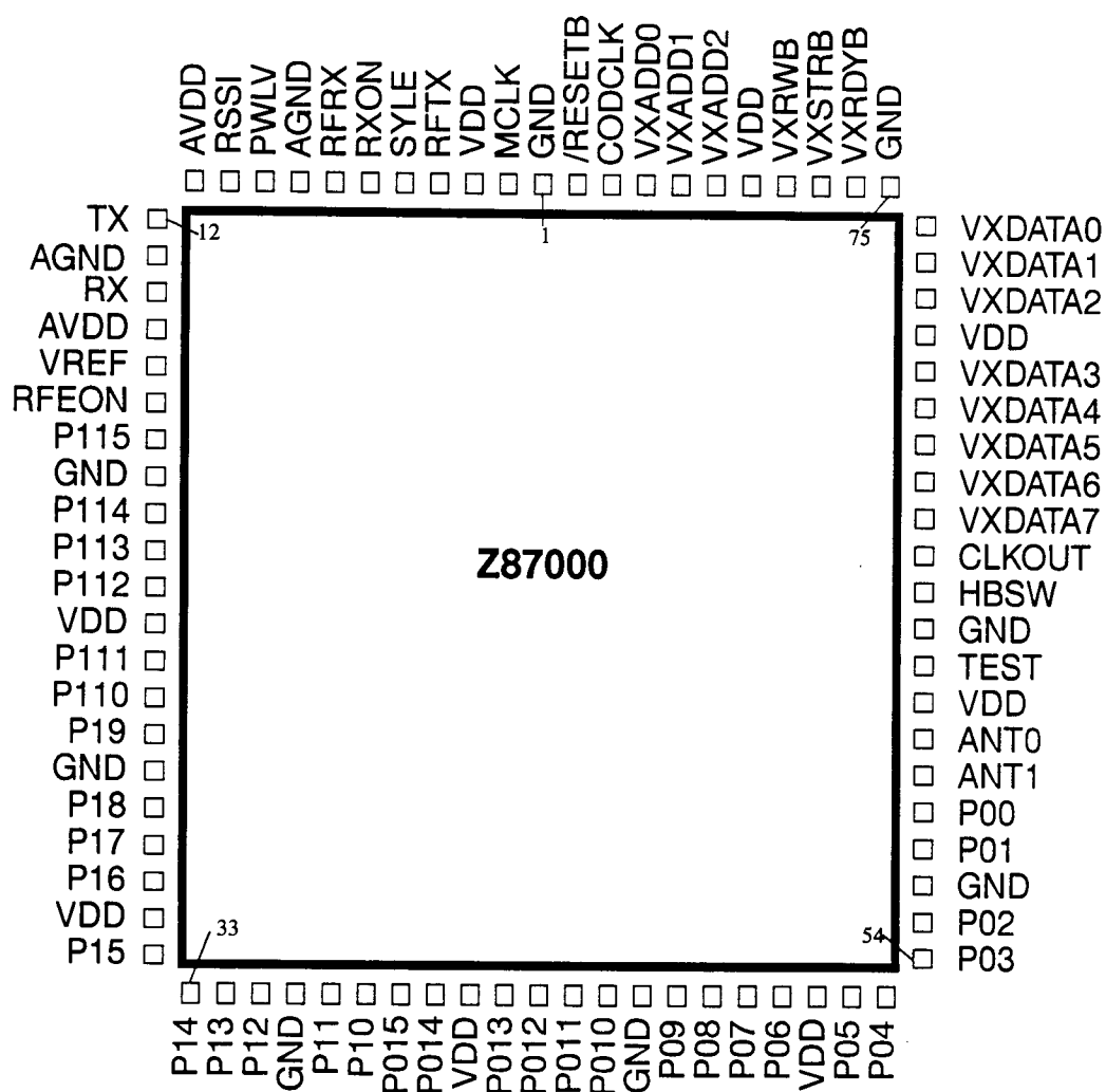
Figure 3. 84-Pin PLCC ROM Pin Configuration (Z87000 only)
