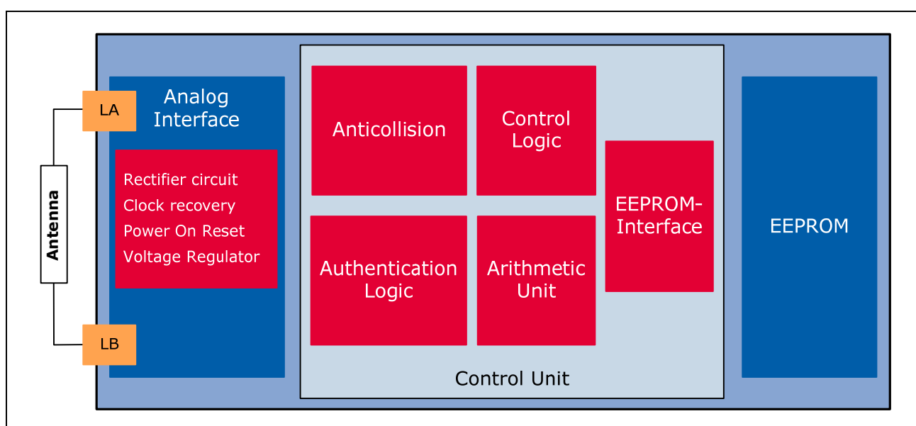
Figure 6 Block Diagram
