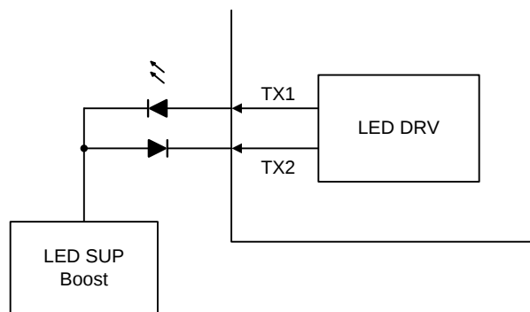
H-Bridge Mode
