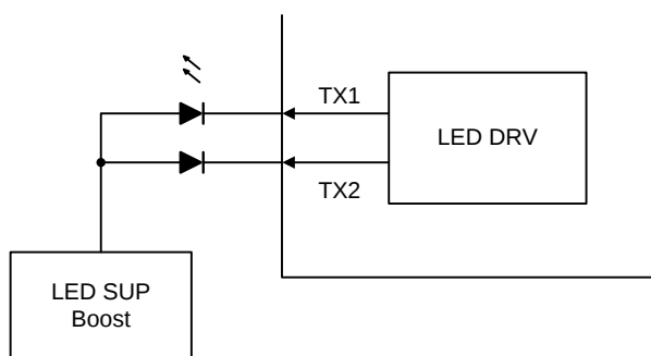
Push-Pull Mode
