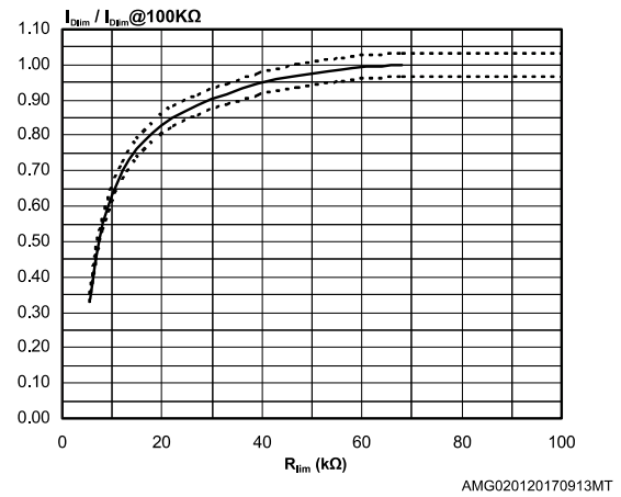
Figure 14: I_{DIM} vs R_{LIM}
