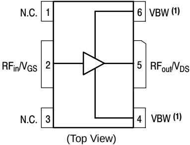
Figure 1. Pin Connections
