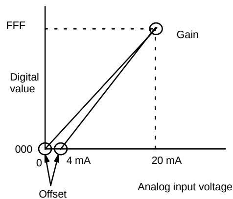
Current Inputs
