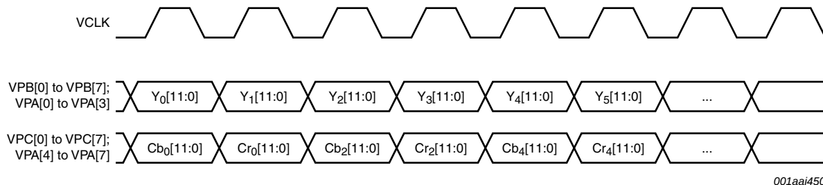
Fig 12. Pixel encoding YCbCr 4 : 2 : 2 semi-planar embedded synchronization input (rising edge)
