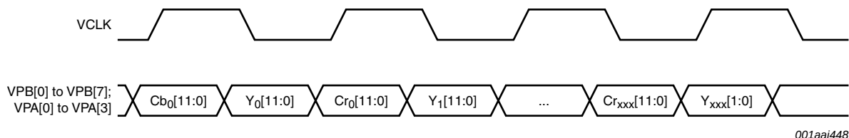
Fig 10. Pixel encoding YCbCr 4 : 2 : 2 ITU656-like embedded synchronization input (double edge)
