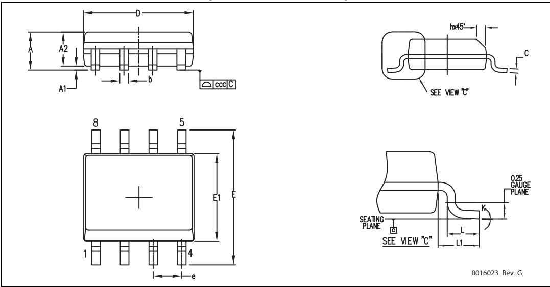
Figure 14. SO-8 drawings
