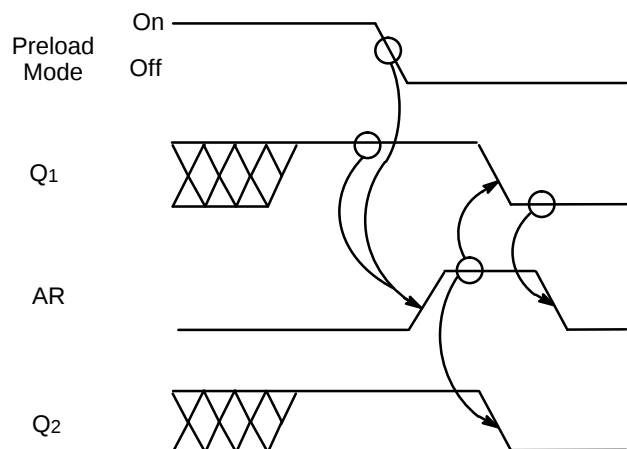
Figure 2. Preload/Reset Conflict
