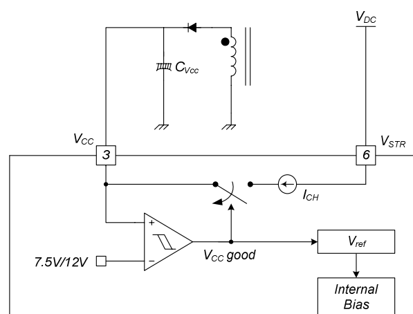
Figure 17. Startup Block
