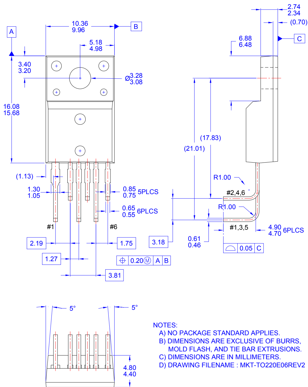
Figure 28. TO-220F-6L (L-Forming)
