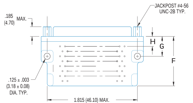
VIEW SHOWN IS FOR 31, 37, AND 51 ARRANGEMENTS
