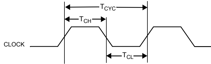
Figure 28-2. GPIO Timing Diagram
