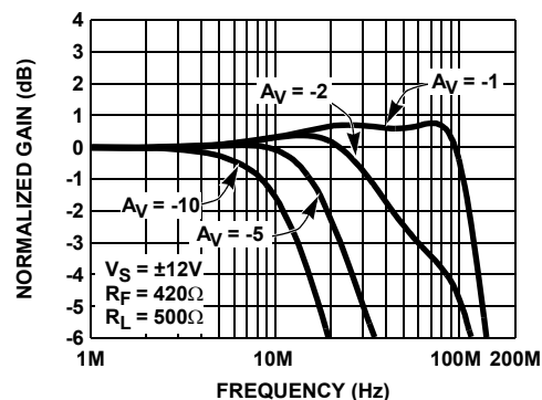
FIGURE 4. INVERTING FREQUENCY RESPONSE (GAIN)
