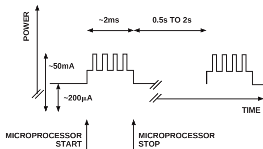
Figure 17. Digital Power as a Function of Time
