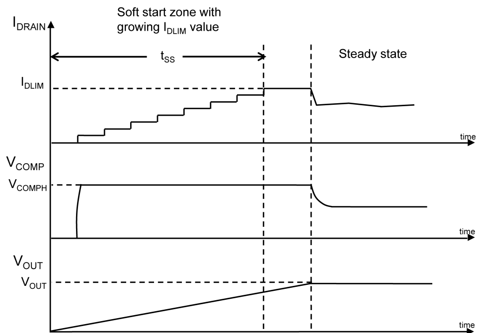
Figure 27. Soft startup
