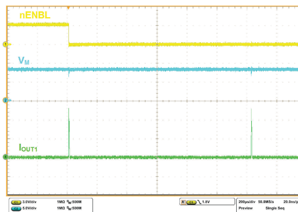
Figure 8-5. OCP Separated by t_{RETRY} With V_M = 8.2 V and OUT1 Shorted to V_M
