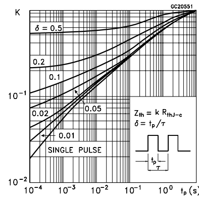
Figure 5. Thermal impedance for TO-220
