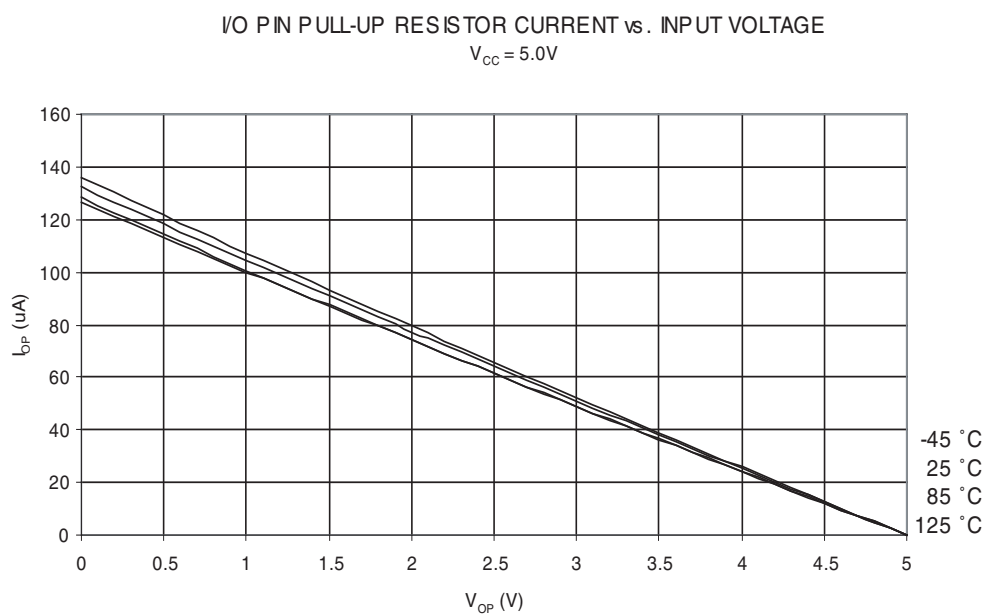
Figure 30-16. I/O pin Pull-up Resistor Current vs. Input Voltage ( V_{CC} = 5V )
