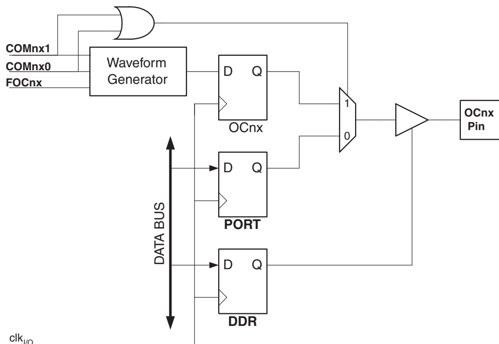
Figure 21-5. Compare Match Output Unit, Schematic
