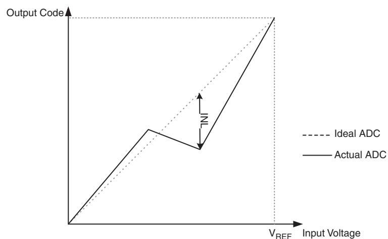
Figure 25-11. Integral Non-linearity (INL)
