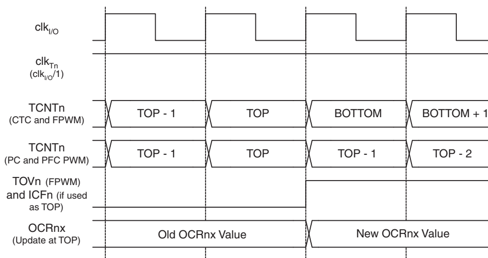
Figure 21-12. Timer/Counter Timing Diagram, no Prescaling
