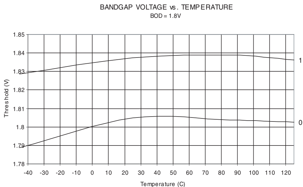
Figure 30-31. BOD Threshold vs. Temperature (BODLEVEL is 1.8V)
