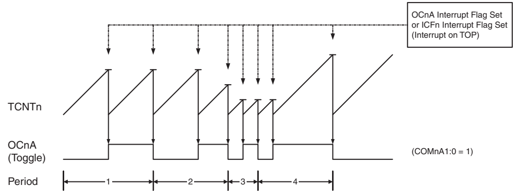
Figure 21-6. CTC Mode, Timing Diagram
