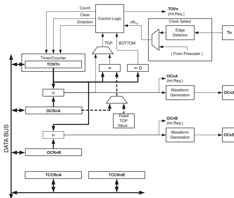
Figure 20-1. 8-bit Timer/Counter Block Diagram
