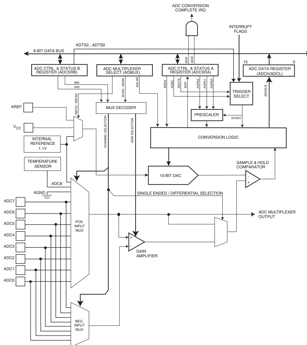
Figure 25-1. Analog to Digital Converter Block Schematic
