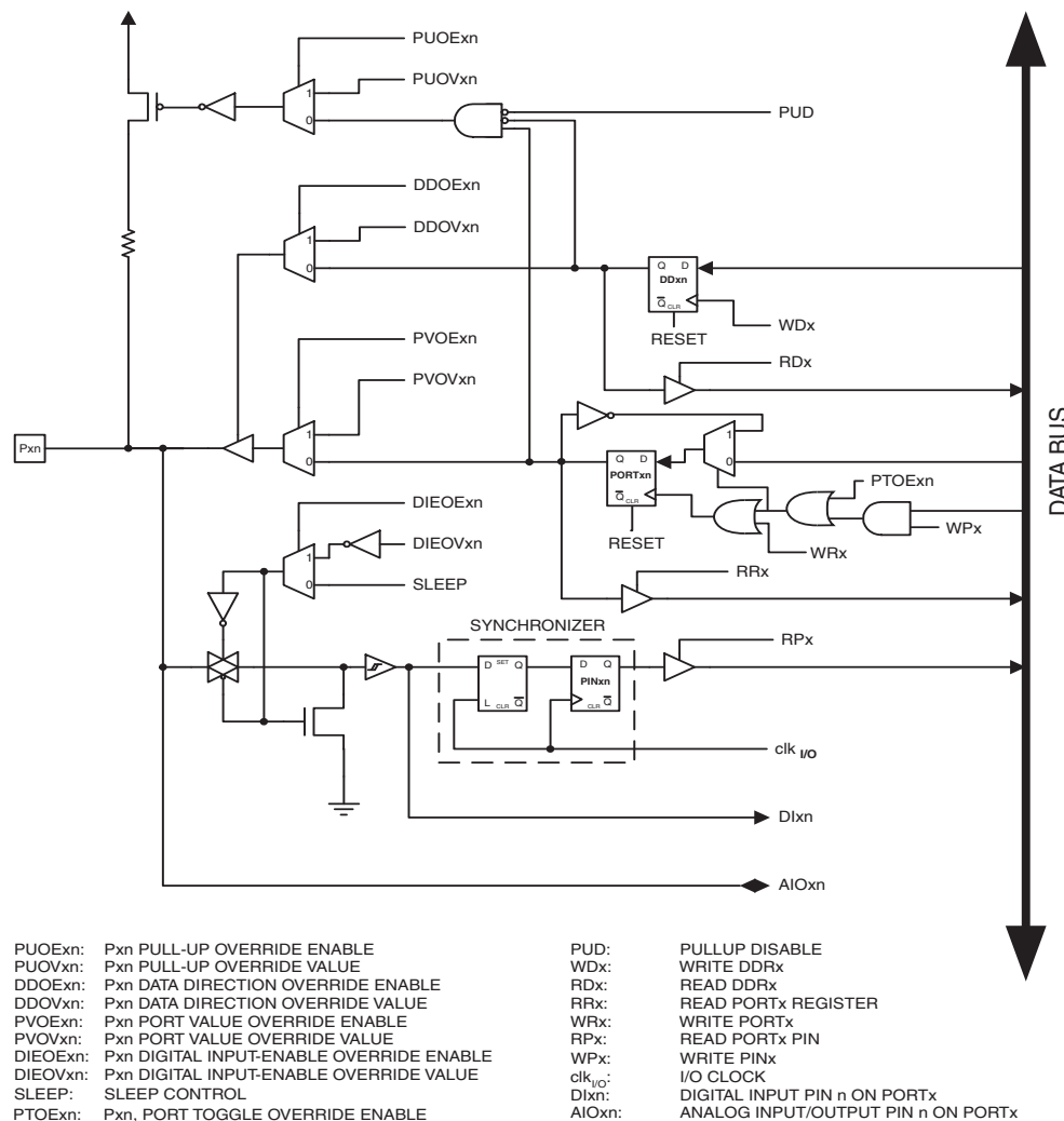
Figure 19-5. Alternate Port Functions (1)
