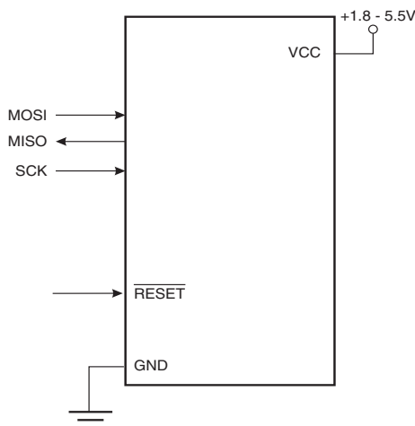
Figure 28-1. Serial Programming and Verify (1)
