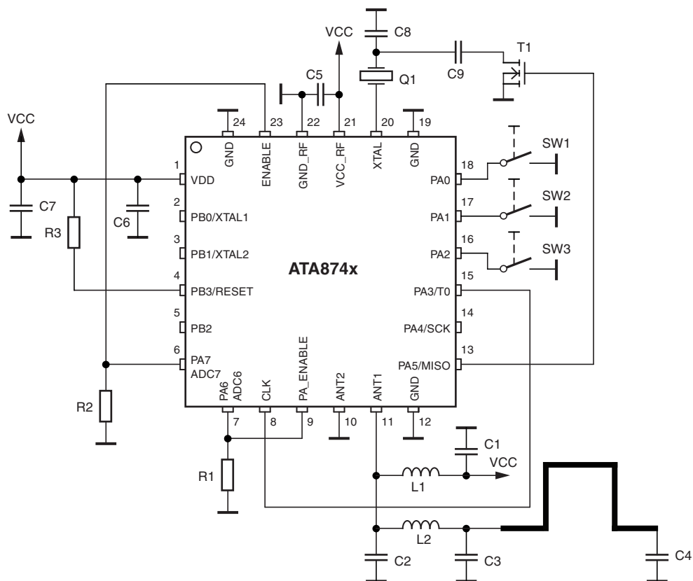
Figure 8-3. Typical FSK Application ATA8743
