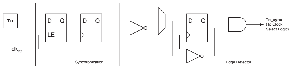
Figure 22-1. T_0 Pin Sampling
