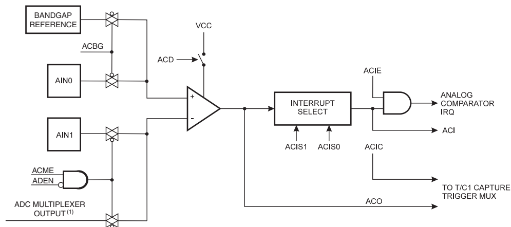
Figure 24-1. Analog Comparator Block Diagram (1)
