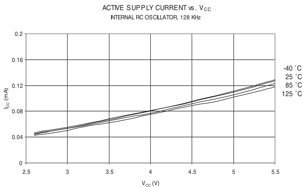
Figure 30-7. Active Supply Current vs. V_{CC} (Internal RC Oscillator, 128 kHz)
