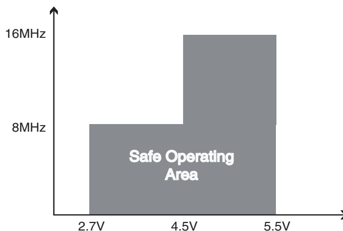
Figure 29-1. Maximum Frequency vs. V_{CC}
