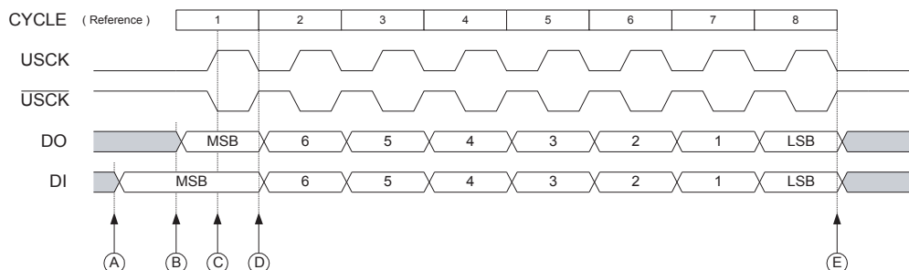
Figure 23-3. Three-wire Mode, Timing Diagram
