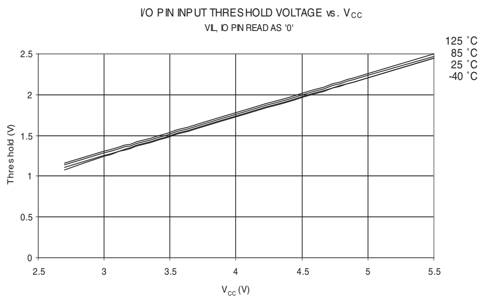
Figure 30-24. I/O Pin Input threshold Voltage vs. V_{CC} ( V_{IL} , IO Pin Read as '0')
