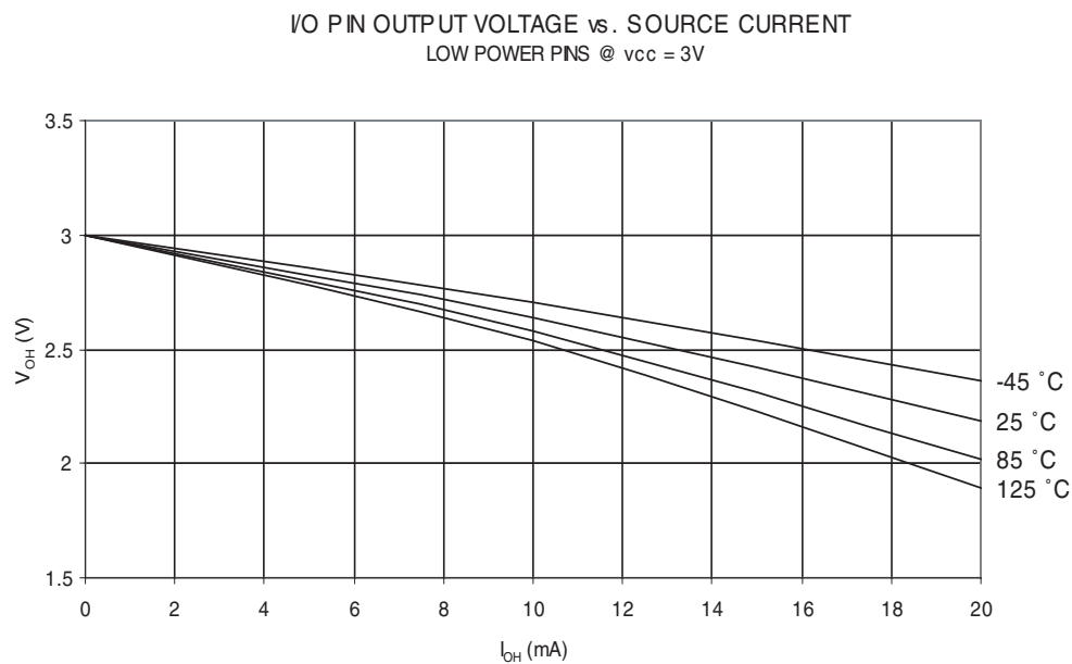
Figure 30-21. I/O Pin Output Voltage vs. Source Current ( V_{CC} = 3V )
