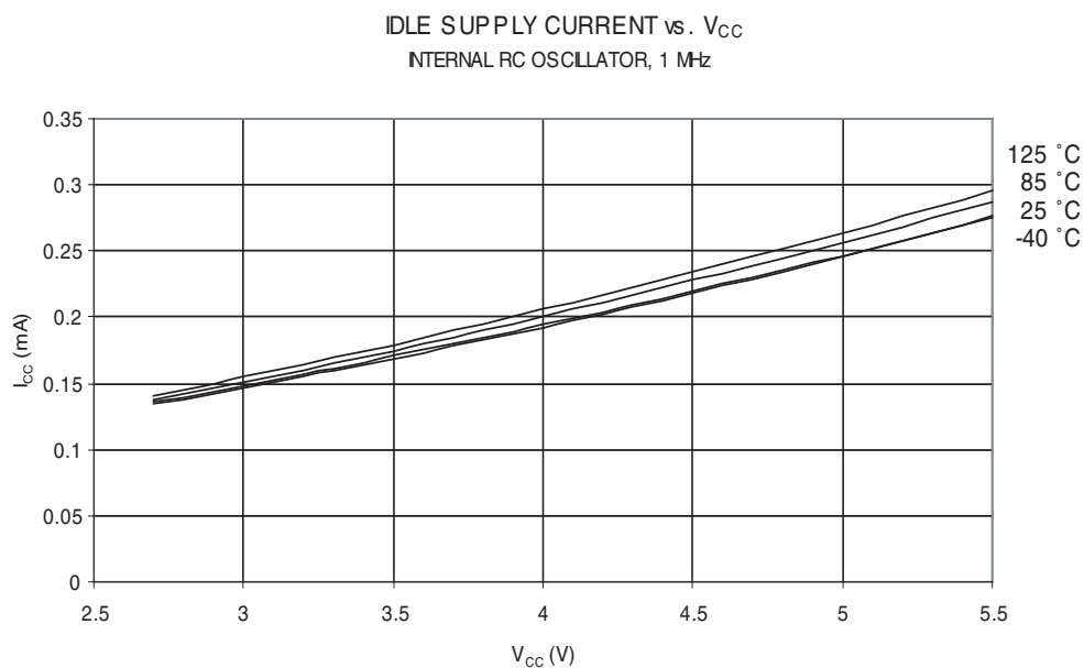
Figure 30-11. Idle Supply Current vs. V_{CC} (Internal RC Oscillator, 1 MHz)
