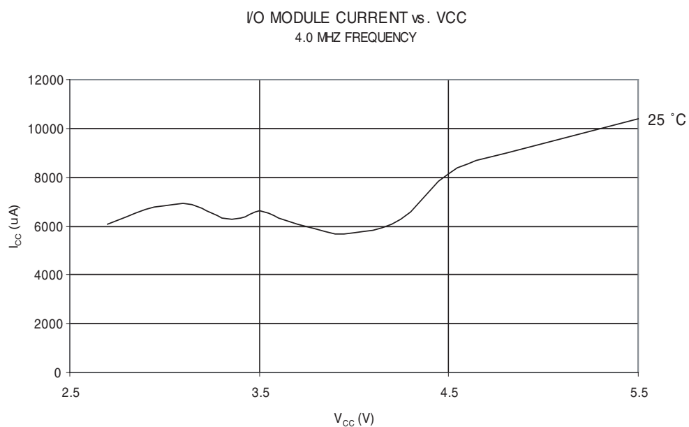
Figure 30-39. Programming Current vs. V_{CC}
