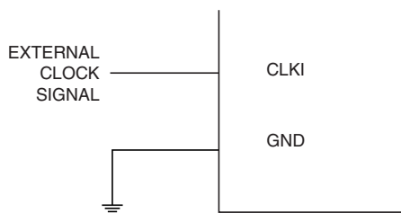
Figure 14-3. External Clock Drive Configuration
