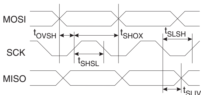
Figure 29-3. Serial Programming Timing
