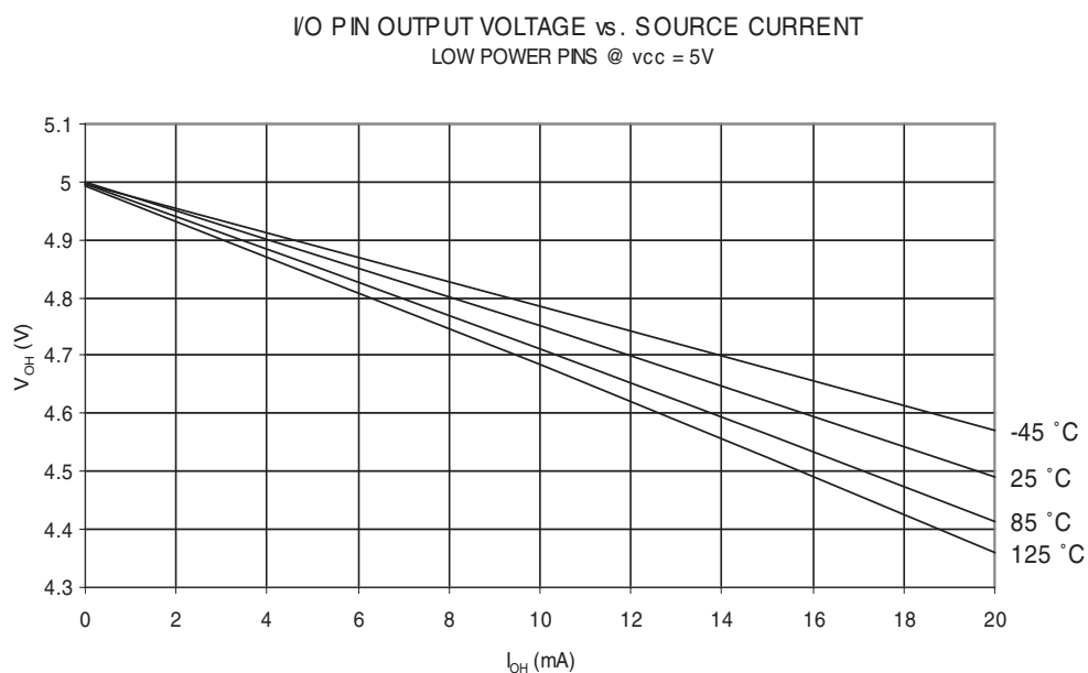
Figure 30-22. I/O Pin output Voltage vs. Source Current ( V_{CC} = 5V )
