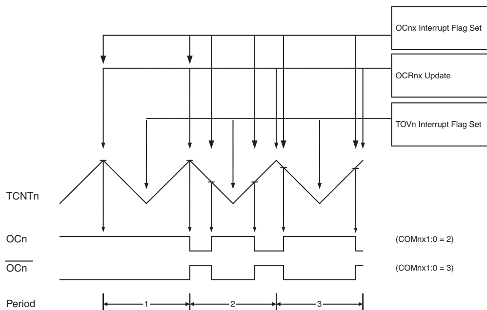
Figure 20-7. Phase Correct PWM Mode, Timing Diagram
