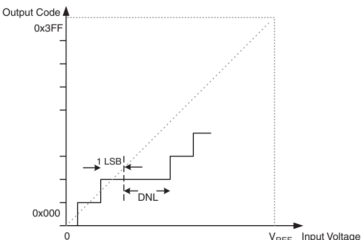
Figure 25-12. Differential Non-linearity (DNL)
