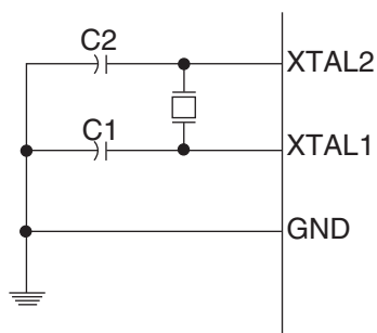
Figure 14-2. Crystal Oscillator Connections
