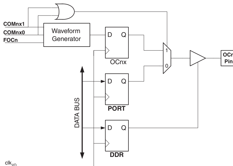
Figure 20-4. Compare Match Output Unit, Schematic
