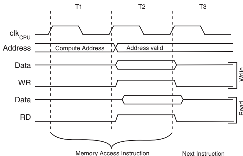
Figure 13-3. On-chip Data SRAM Access Cycles
