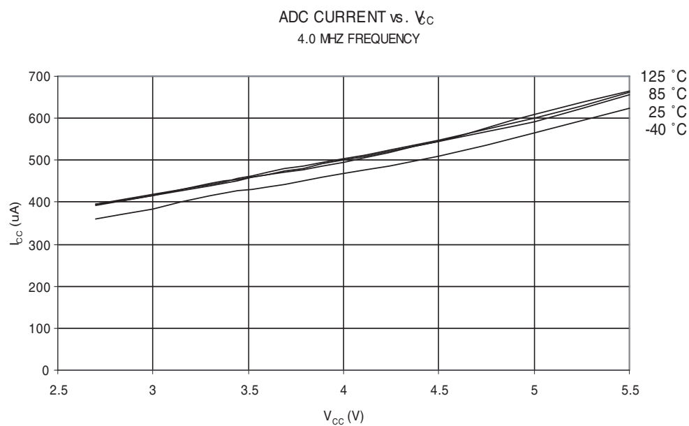
Figure 30-36. ADC Current vs. V CC
