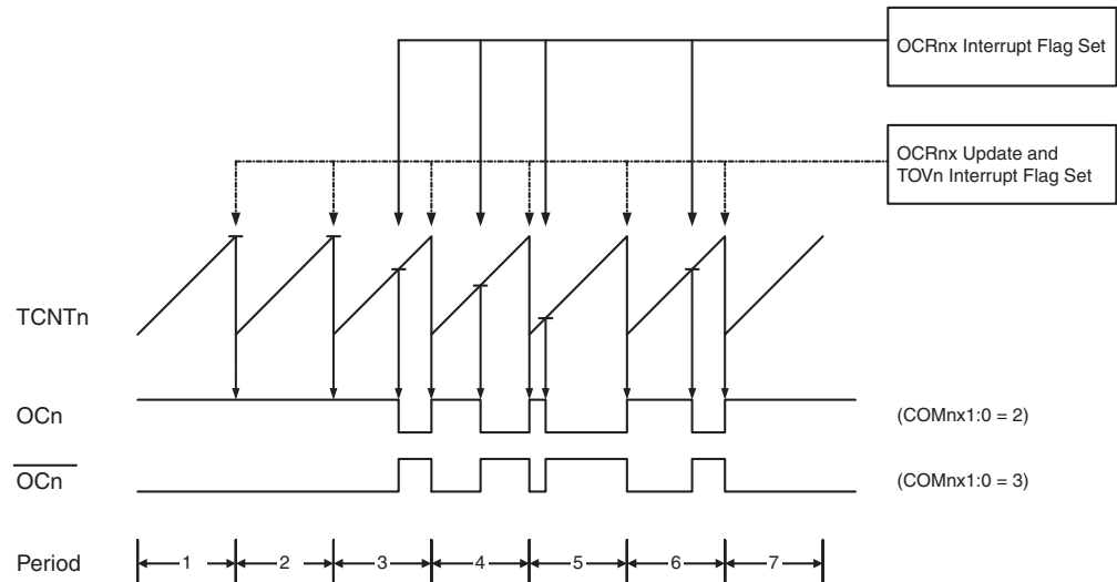
Figure 20-6. Fast PWM Mode, Timing Diagram
