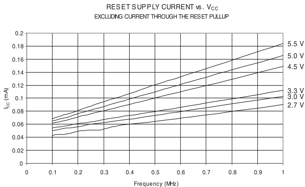
Figure 30-42. Reset Supply Current vs. V_{CC} (0.1 - 1.0 MHz, excluding Current Through the Reset Pull-up)
