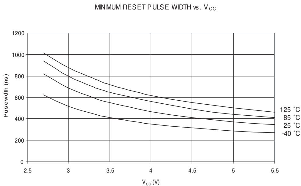
Figure 30-44. Minimum Reset Pulse Width vs. V_{CC}
