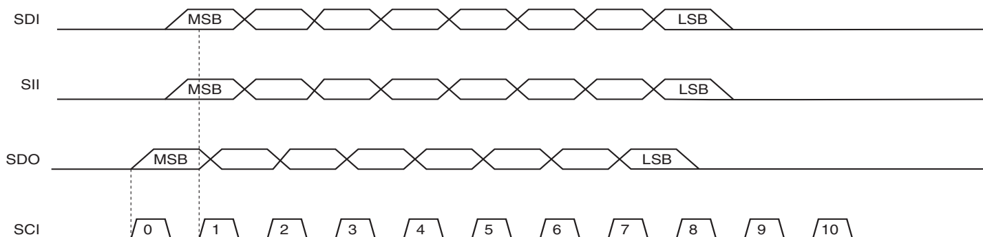
Figure 28-5. High-voltage Serial Programming Waveforms
