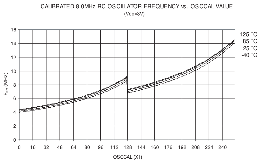
Figure 30-35. Calibrated 8 MHz RC Oscillator Frequency vs. OSCCAL Value
