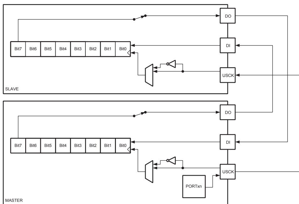
Figure 23-2. Three-wire Mode Operation, Simplified Diagram
