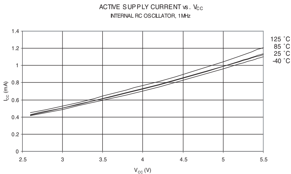
Figure 30-6. Active Supply Current vs. V_{CC} (Internal RC Oscillator, 1 MHz)
