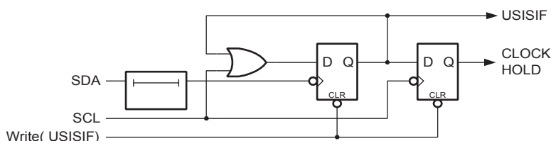
Figure 23-6. Start Condition Detector, Logic Diagram
