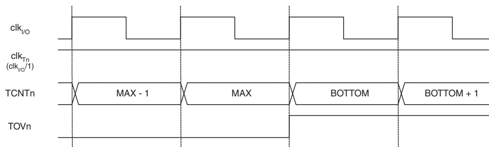
Figure 20-8. Timer/Counter Timing Diagram, no Prescaling
