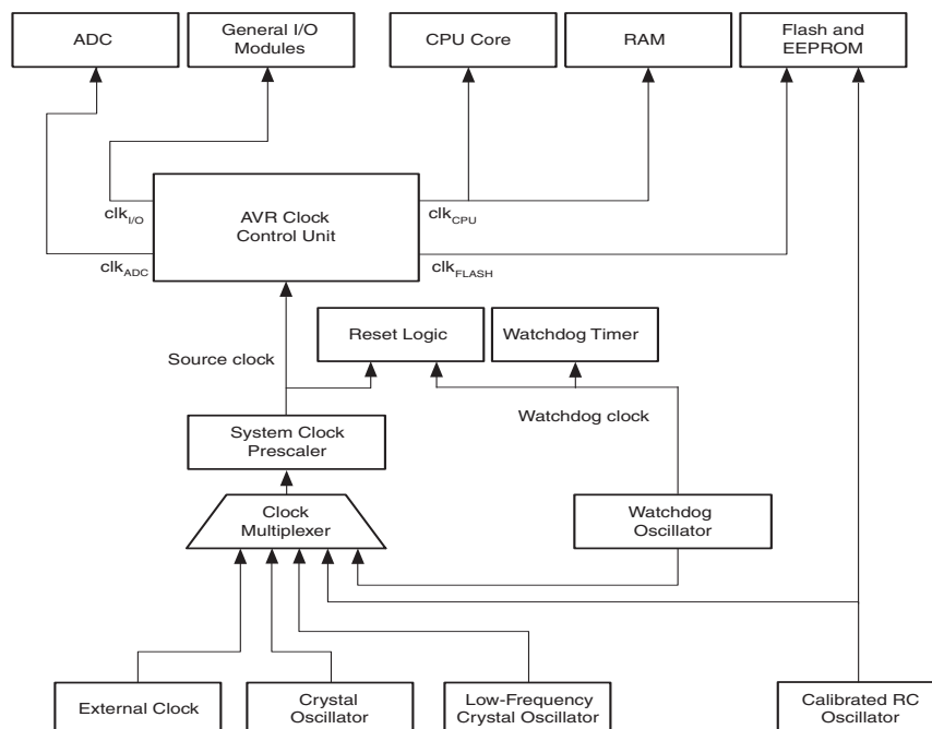
Figure 14-1. Clock Distribution
