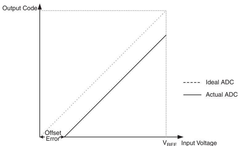
Figure 25-9. Offset Error
