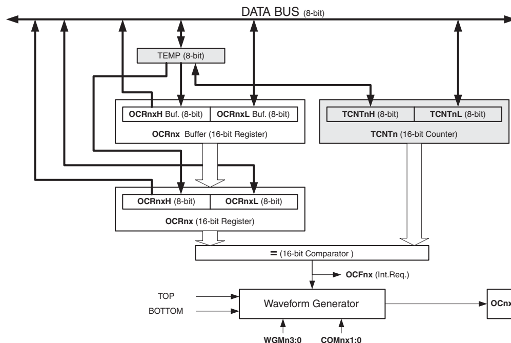
Figure 21-4. Output Compare Unit, Block Diagram
