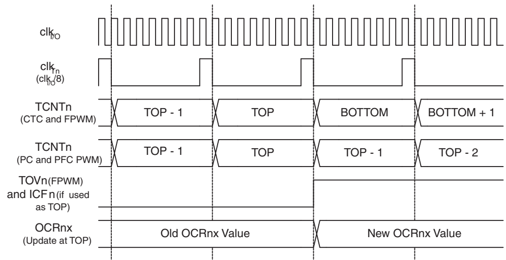
Figure 21-13. Timer/Counter Timing Diagram, with Prescaler ( f_{clk\_I/O}/8 )
