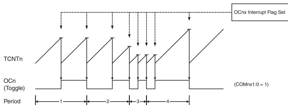
Figure 20-5. CTC Mode, Timing Diagram
