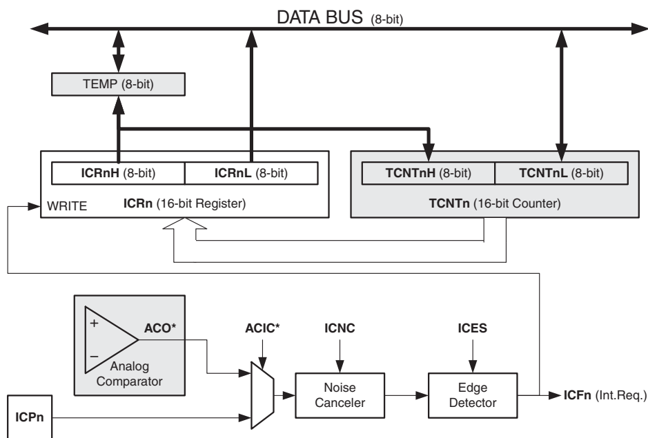
Figure 21-3. Input Capture Unit Block Diagram
