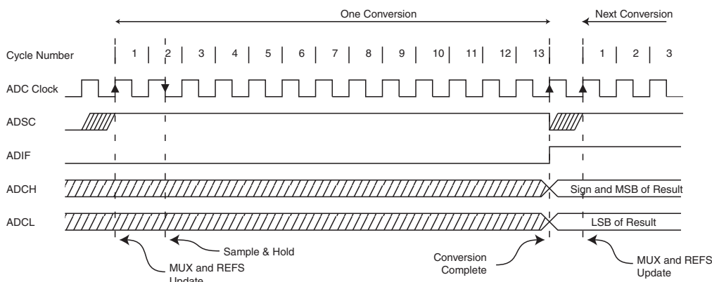
Figure 25-5. ADC Timing Diagram, Single Conversion
