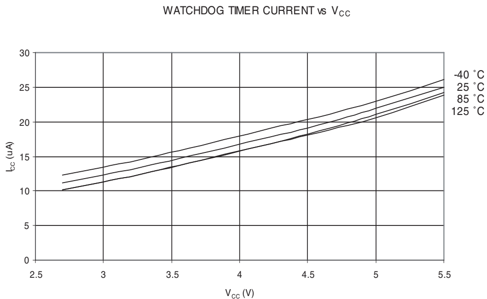
Figure 30-41. Watchdog Timer Current vs. V_{CC}
