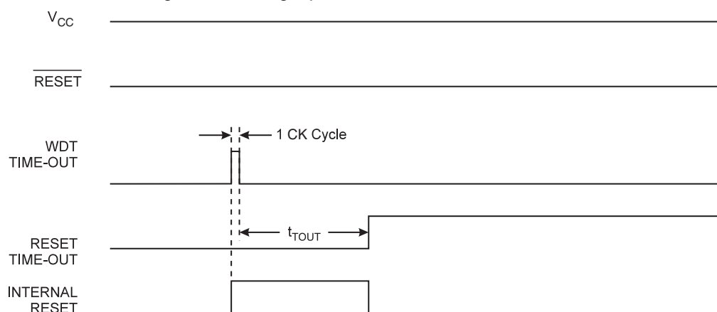
Figure 16-6. Watchdog Reset During Operation
