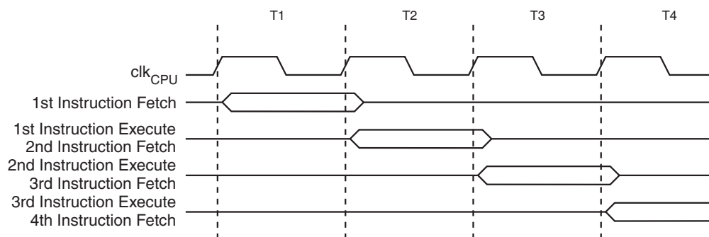
Figure 12-4. The Parallel Instruction Fetches and Instruction Executions
