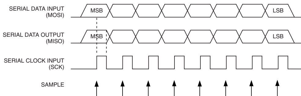
Figure 29-4. Serial Programming Waveforms
