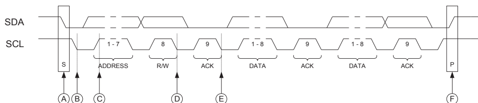
Figure 23-5. Two-wire Mode, Typical Timing Diagram
