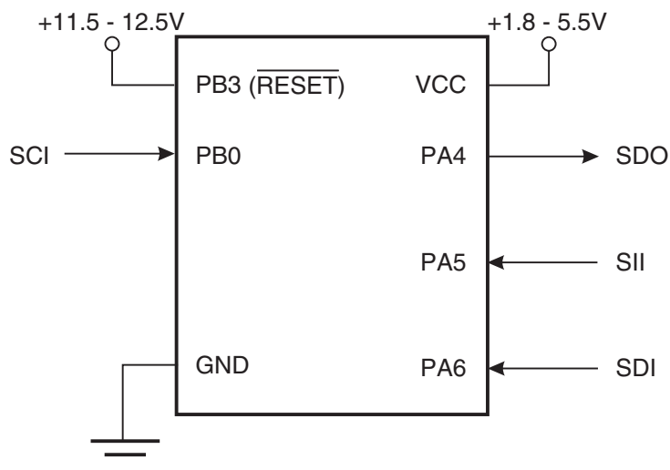
Figure 28-3. High-voltage Serial Programming
