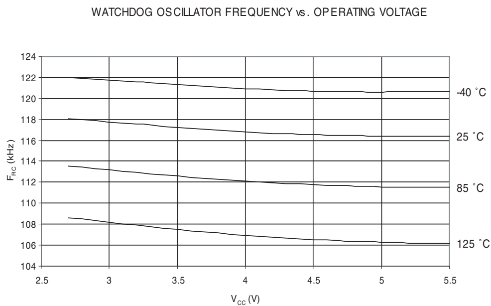
Figure 30-32. Watchdog Oscillator Frequency vs. V_{CC}
