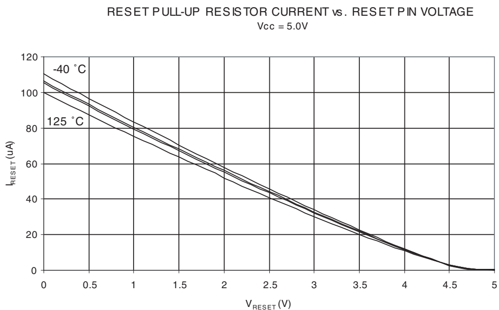
Figure 30-18. Reset Pull-up Resistor Current vs. Reset Pin Voltage ( V_{CC} = 5V )
