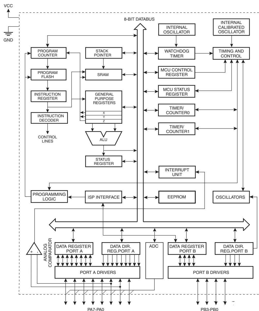
Figure 9-1. Block Diagram
