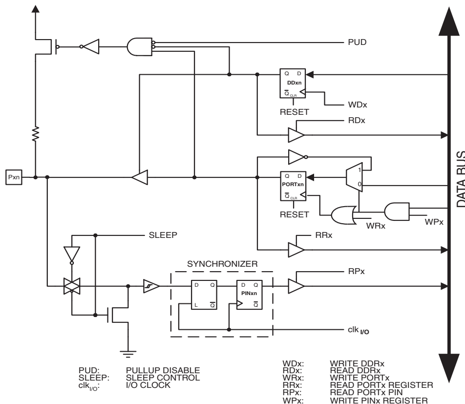
Figure 19-2. General Digital I/O (1)
