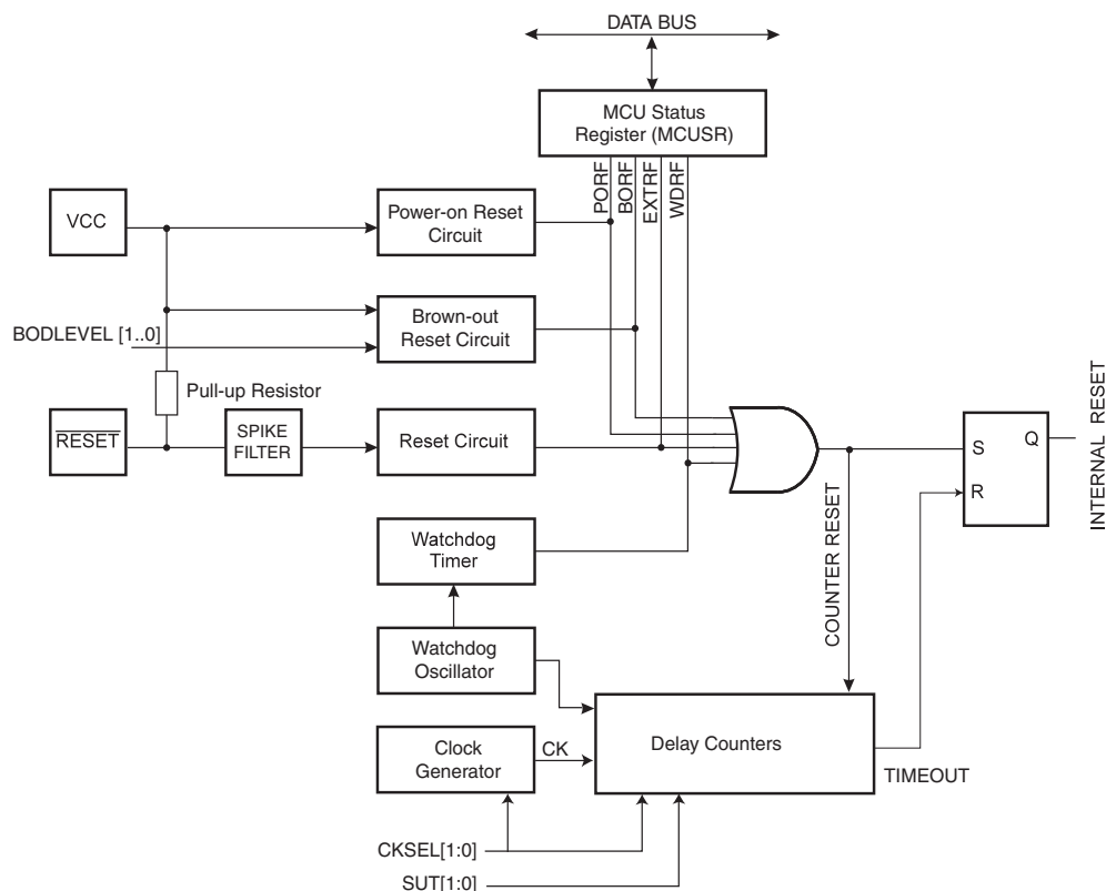
Figure 16-1. Reset Logic
