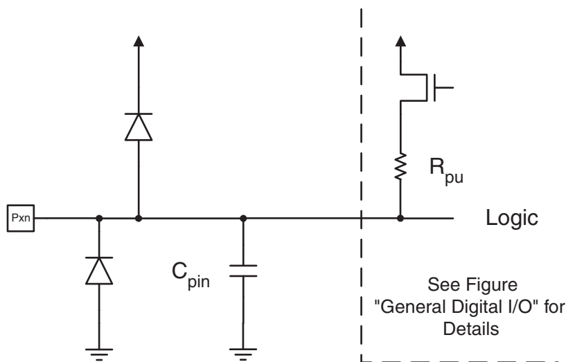
Figure 19-1. I/O Pin Equivalent Schematic
