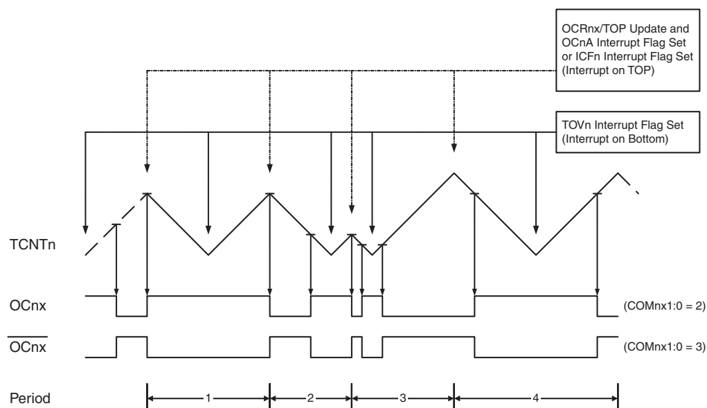
Figure 21-8. Phase Correct PWM Mode, Timing Diagram
