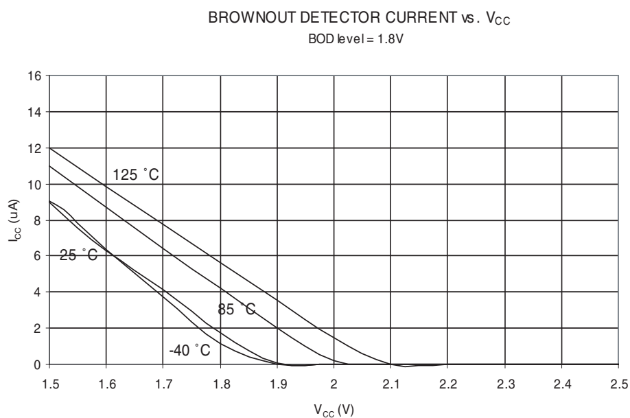
Figure 30-40. Brownout Detector Current vs. V_{CC}
