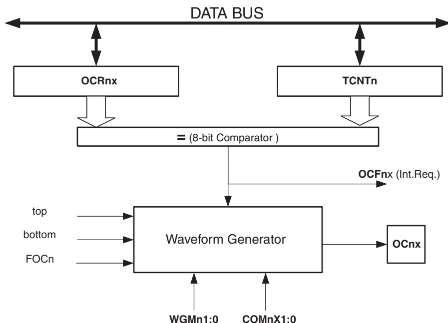
Figure 20-3. Output Compare Unit, Block Diagram
