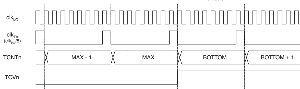
Figure 20-9. Timer/Counter Timing Diagram, with Prescaler ( f_{clk\_I/O}/8 )
