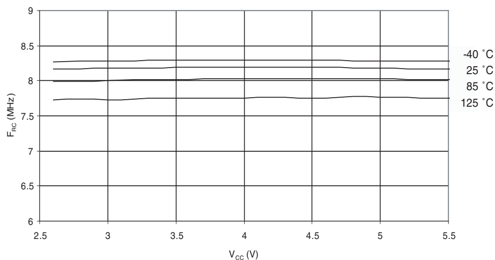
Figure 30-34. Calibrated 8 MHz RC oscillator Frequency vs. Temperature
