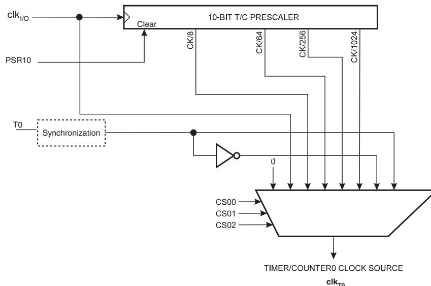
Figure 22-2. Prescaler for Timer/Counter0
