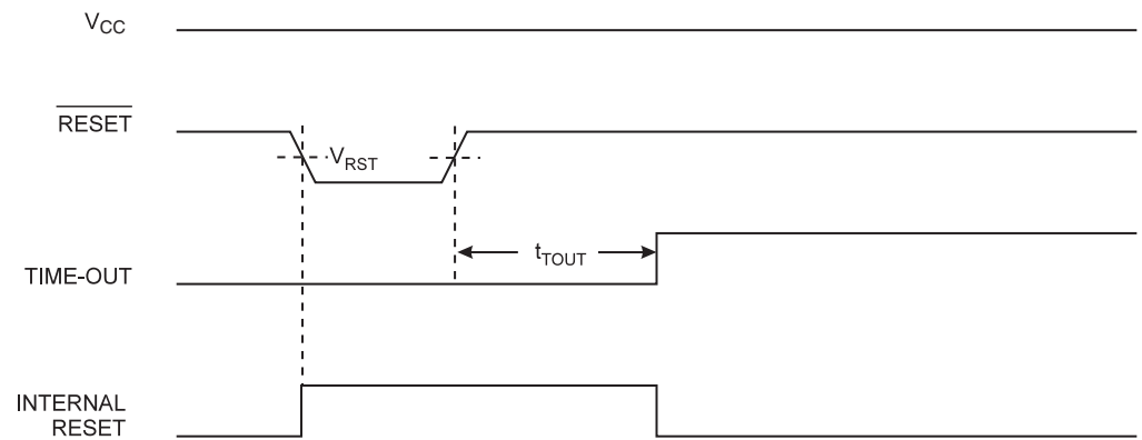
Figure 16-4. External Reset During Operation
