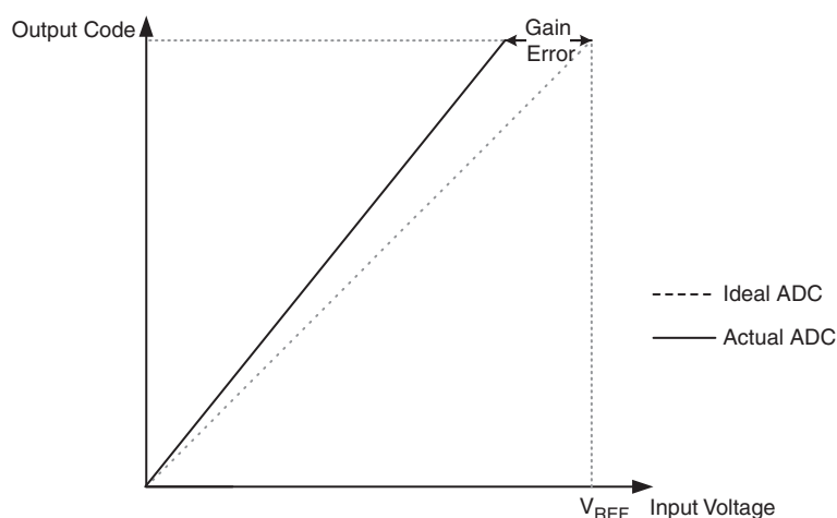
Figure 25-10. Gain Error
