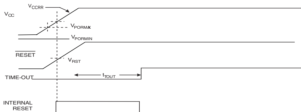
Figure 16-2. MCU Start-up, \overline{\text{RESET}} Tied to V_{CC}
