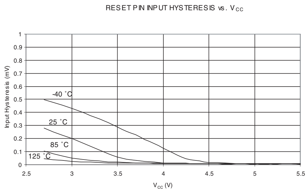
Figure 30-28. Reset Pin Input Hysteresis vs. V_{CC}
