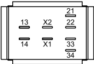
36 Switching element for Pushbutton | Keylock- and Selector switch 2 positions page 36
