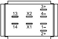
37 PCB plug-in base page 38
