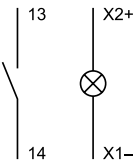
28 Switching element for Pushbutton | Keylock- and Selector switch 2 positions page 36
