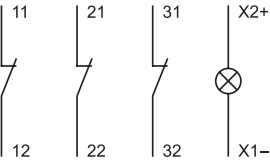
26 Switching element for Pushbutton | Keylock- and Selector switch 2 positions page 36
