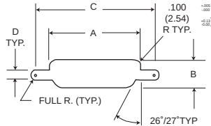
Figure 2 Rear Mounting
