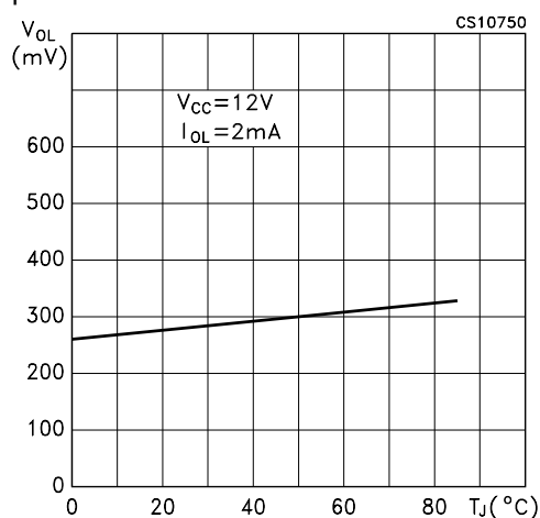
Figure 25 : DSQOUT Pin Logic Low vs Temperature
