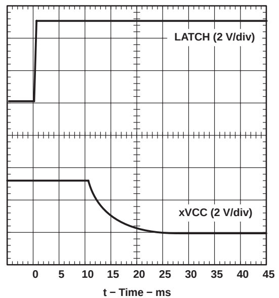
Figure 6. xVCC Propagation Delay and Fall Time With 150- \mu F Load, 3.3-V Switch, V_{I(5V)} = 5\text{ V}
