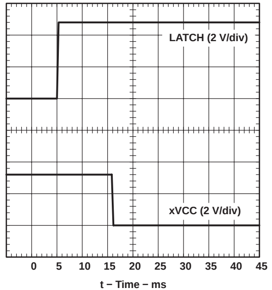
Figure 4. xVCC Propagation Delay and Fall Time With 1- \mu F Load, 3.3-V Switch, ( V_{I(5V)} = 5\text{ V} )
