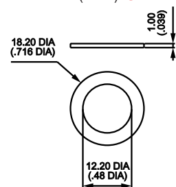
SEALING WASHER Nylon 12mm (.472") U21
