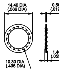
LOCKING RING 1/4 Nickel plated U78 Matte black U93
