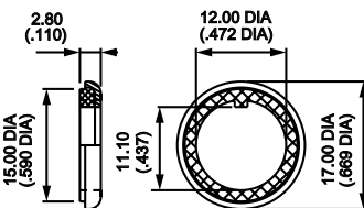
SEALING WASHER U60 15/32
