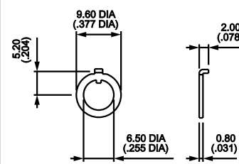
LOCKING RING 1/4 Nickel plated U78 Matte black U93
