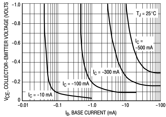
Figure 21. Saturation Region
