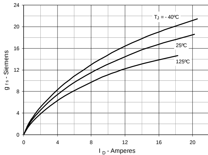
Fig. 9. Transconductance
