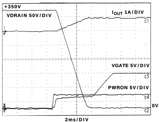
FIGURE 19. +350V LOW SIDE SWITCHING CGATE = 100pF
