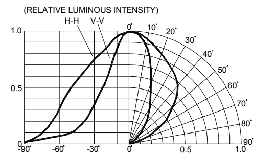
FIG.6 RED & BLUE&GREEN FAR FIELD PATTERN
