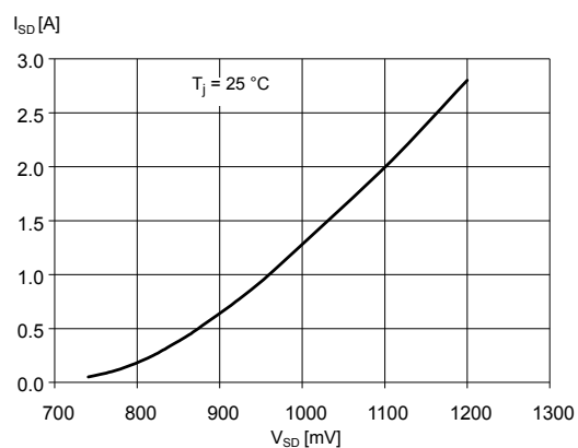
Figure 29. Typical drain-source diode forward ON characteristic
