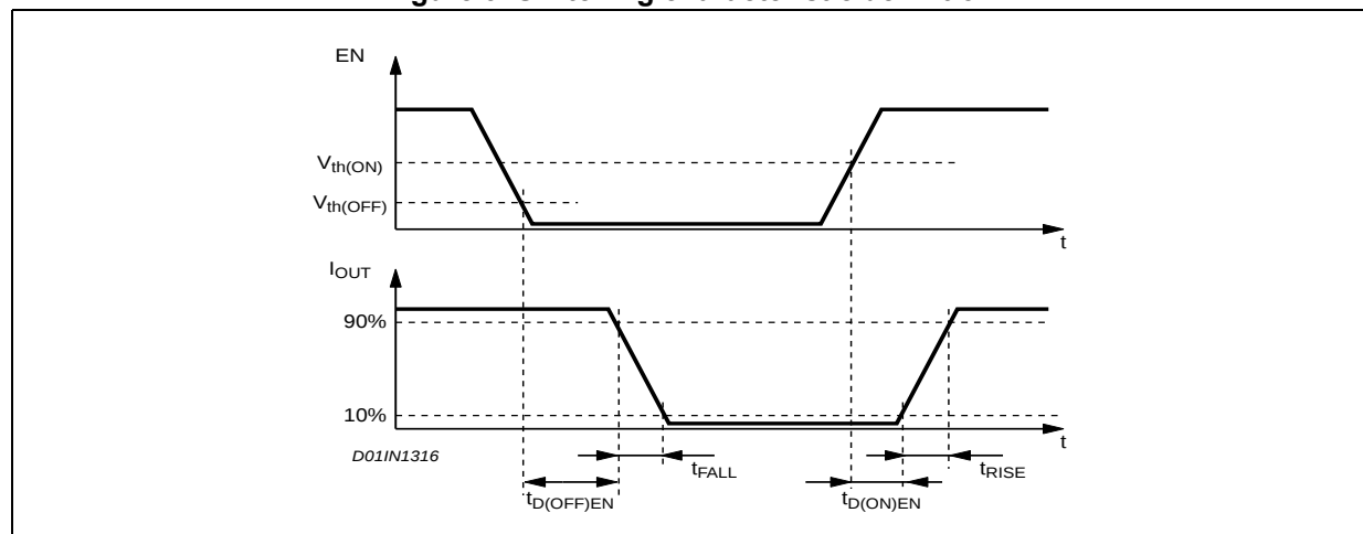
Figure 3. Switching characteristic definition
