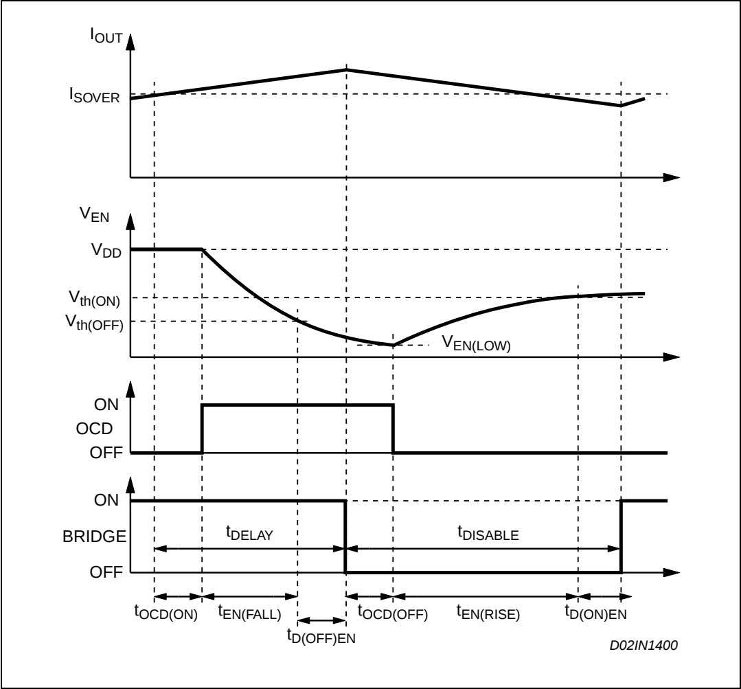
Figure 15. Overcurrent protection waveforms
