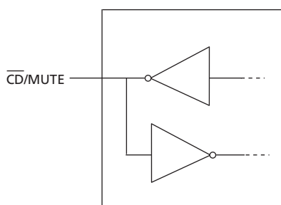
Figure 3-5: \overline{\text{CD}}/\text{MUTE} Circuit
