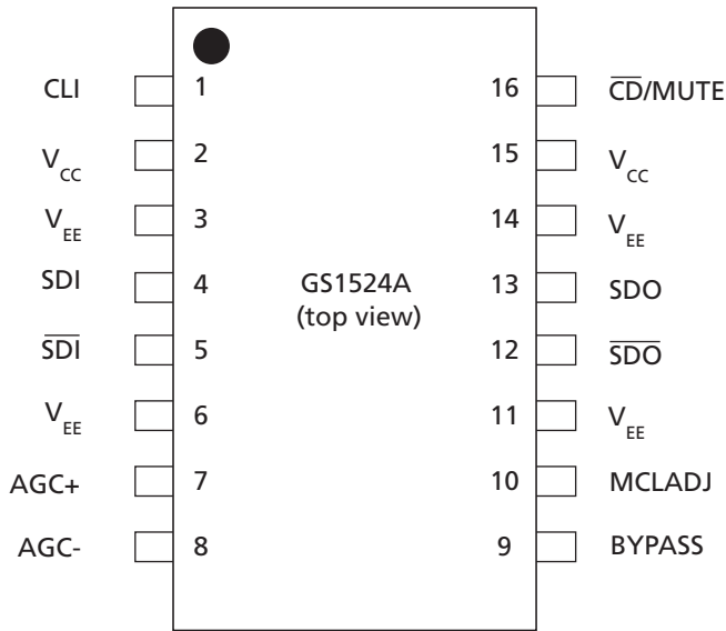
Figure 1-1: 16-Pin SOIC
