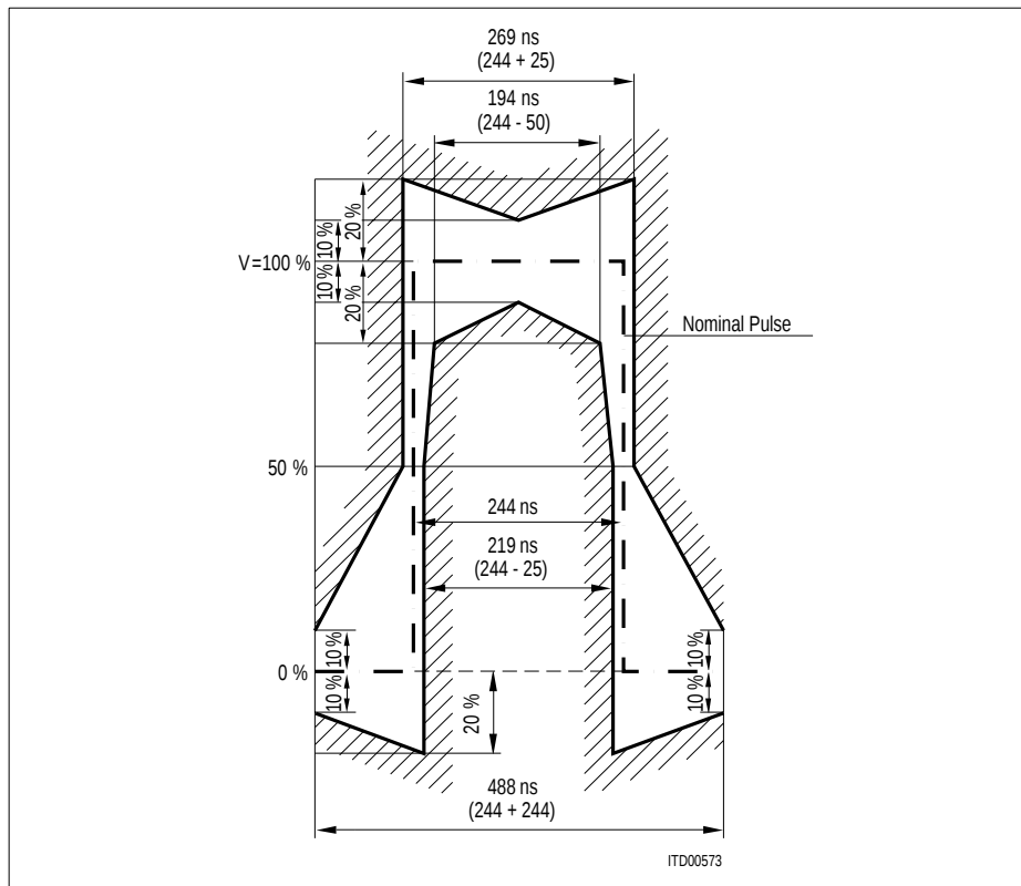
Figure 103 E1 Pulse Shape at Transmitter Output
