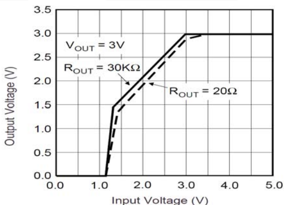
Figure 18. Dropout Characteristics
