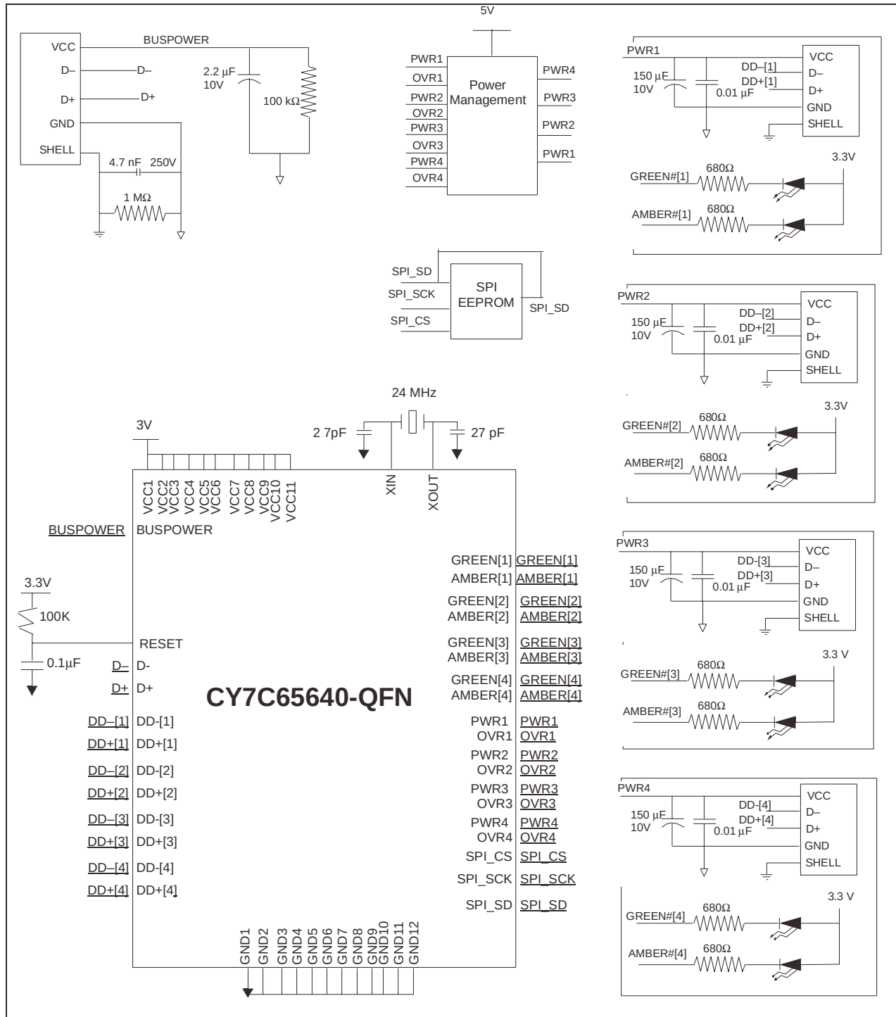
Figure 13-1. Sample Schematic
