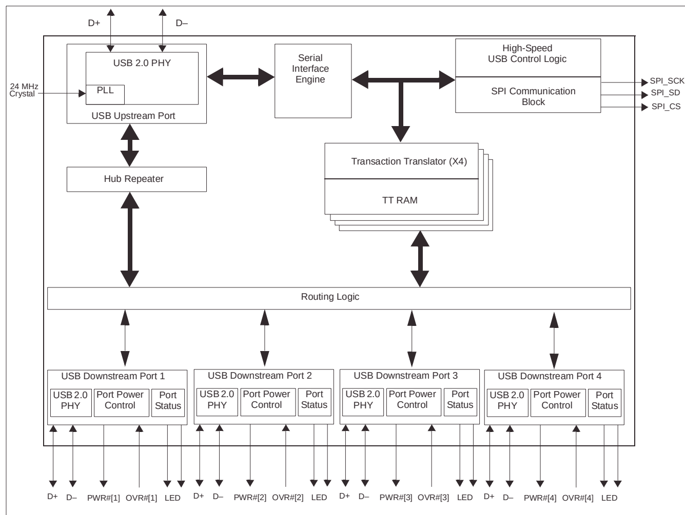
Figure 2-1. Block Diagram
