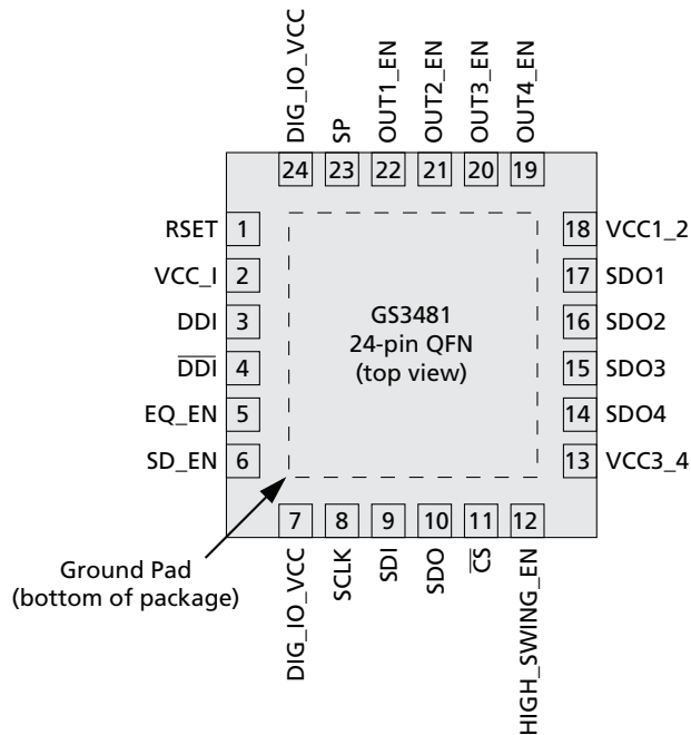
Figure 1-1: Pin Assignment
