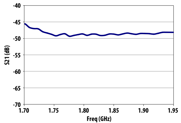
Figure 19d. Rejection plot for (1700 – 1950) MHz
