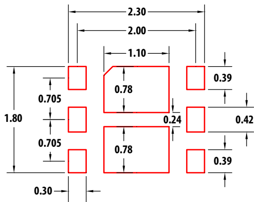
LAND PATTERN
