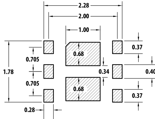
STENCIL OPENING
