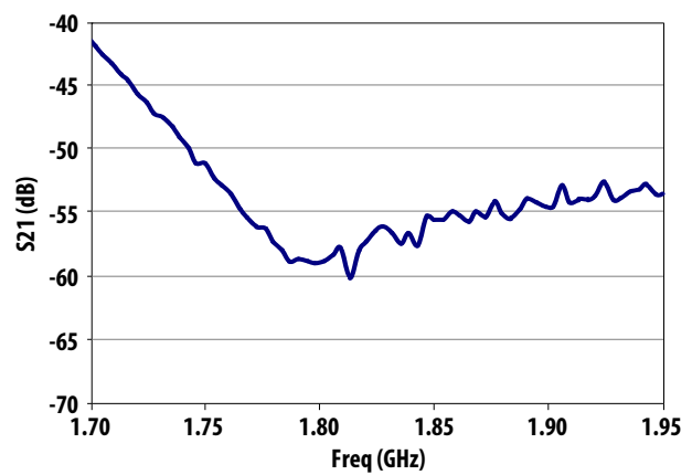
Figure 4d. Rejection plot for (1700 – 1950) MHz
