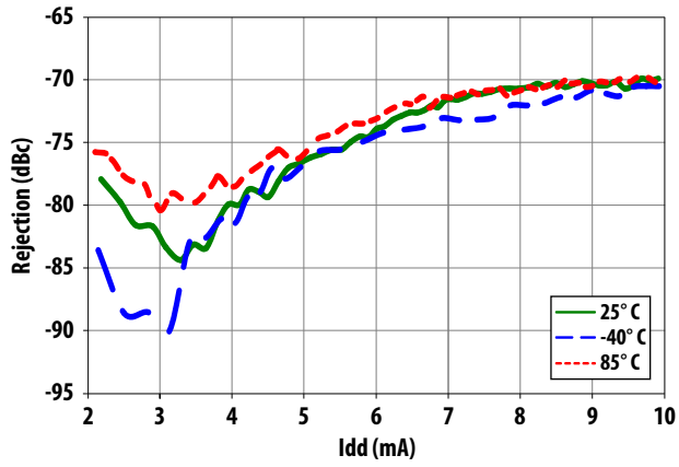
Figure 15. Rejection at 1850 MHz relative to 1.575 GHz vs. Idd
