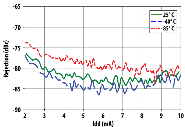
Figure 29. Rejection at 2400 MHz relative to 1.575 GHz vs. Idd
