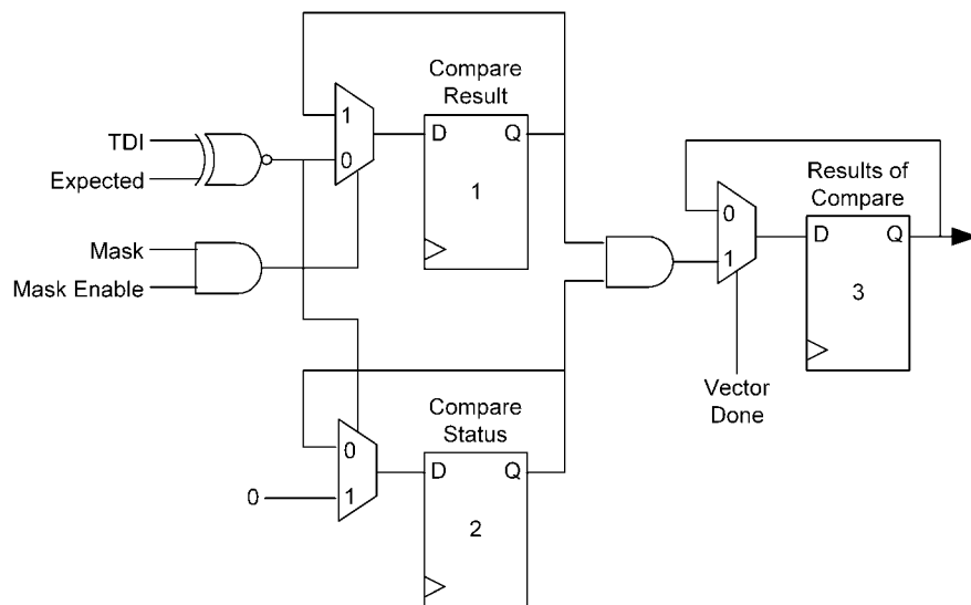
FIGURE 6. Compare Logic
