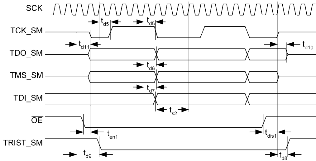
FIGURE 14. SSI Timing Diagram with Clock Divider set to 8
