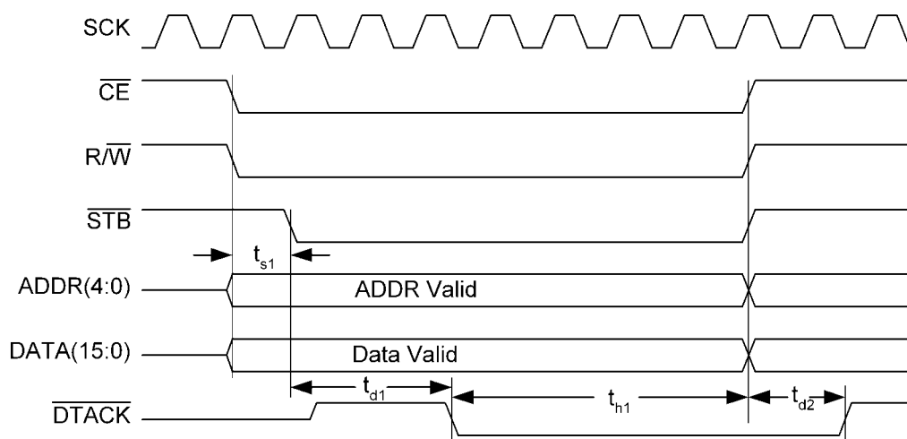
FIGURE 11. PPI Write Cycle Timing Diagram
