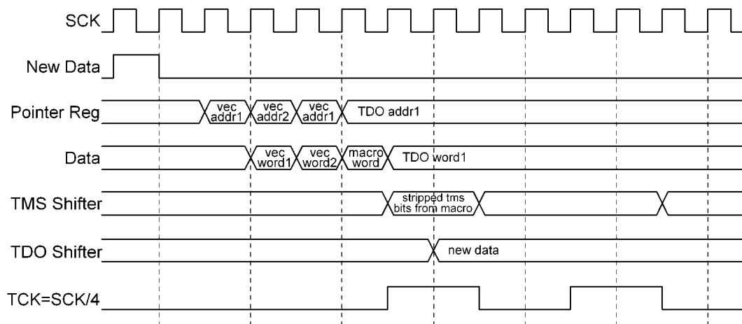
FIGURE 7. Timing from Mode Register Write to Vector Start
