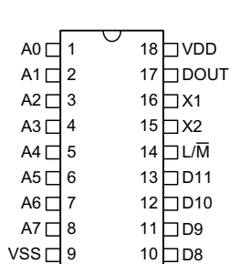
HT12A -18 DIP-A
