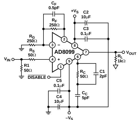
Figure 63. Amplifier Configuration for LFCSP Package, Gain = +2
