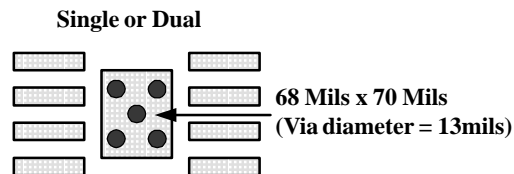
Figure 116. PowerPAD PCB Etch and Via Pattern
