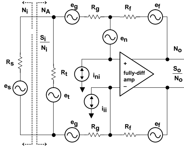
Figure 110. Noise Sources in a Fully Differential Amplifier Circuit
