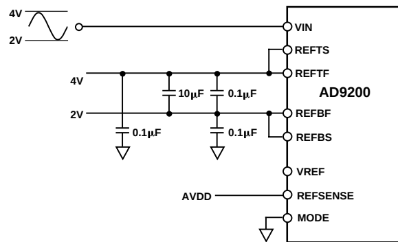
Figure 23a. External Reference ~ 2 V p-p Input Span
