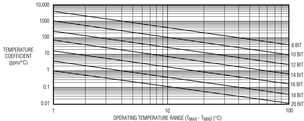
Figure 4. Temperature Coefficient vs. Operating Temperature Range for a 1 LSB Maximum Error
