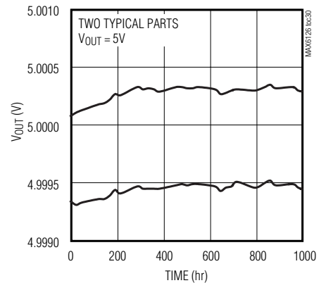
MAX6126B_50 LONG-TERM STABILITY vs. TIME (µMAX)
