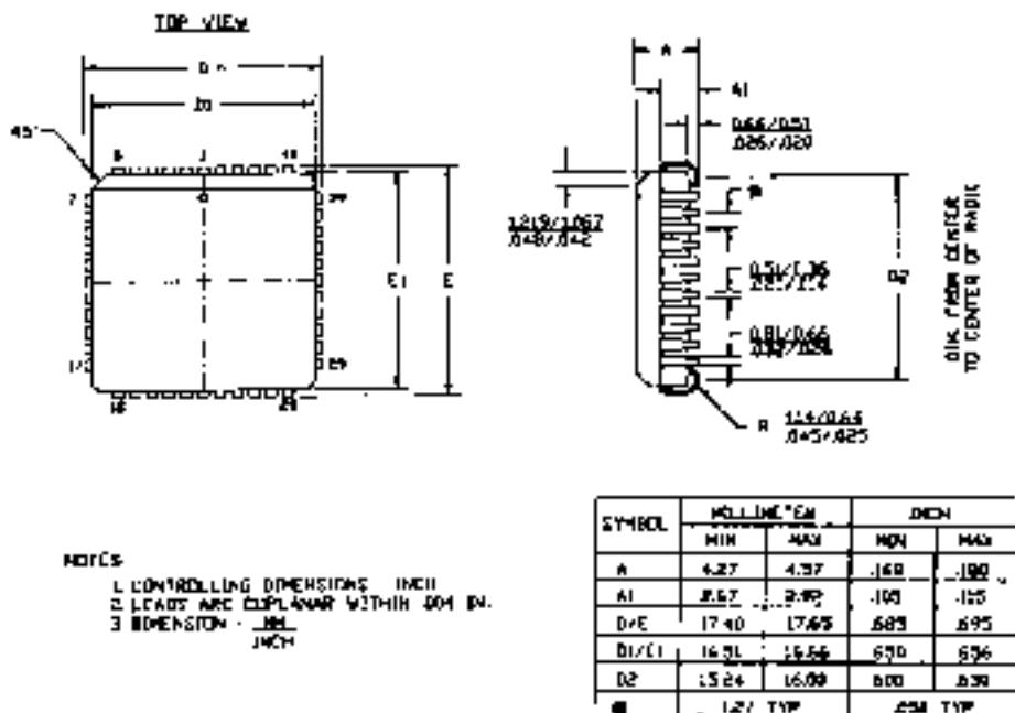
Figure 41. 44-Pin PLC Package Diagram
