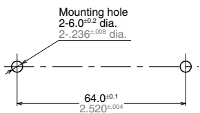
Panel cut-off
