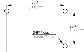
Panel cut-off
