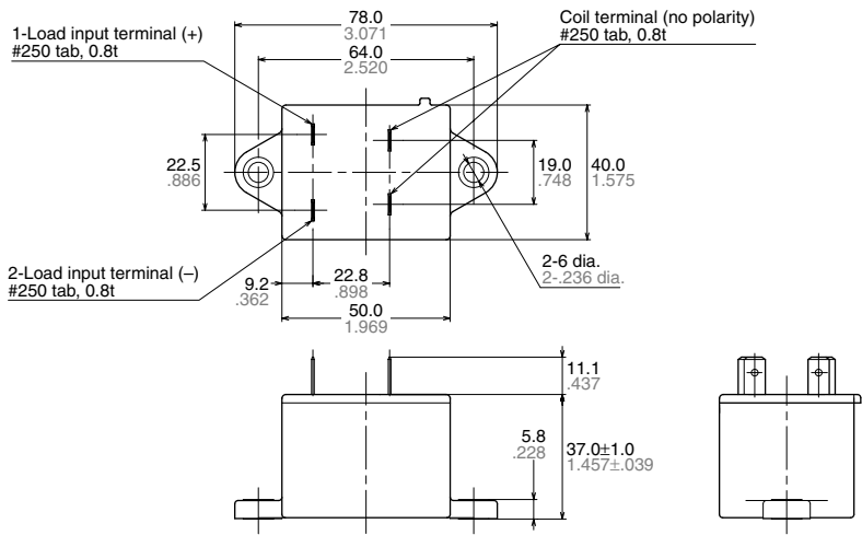
External dimensions
