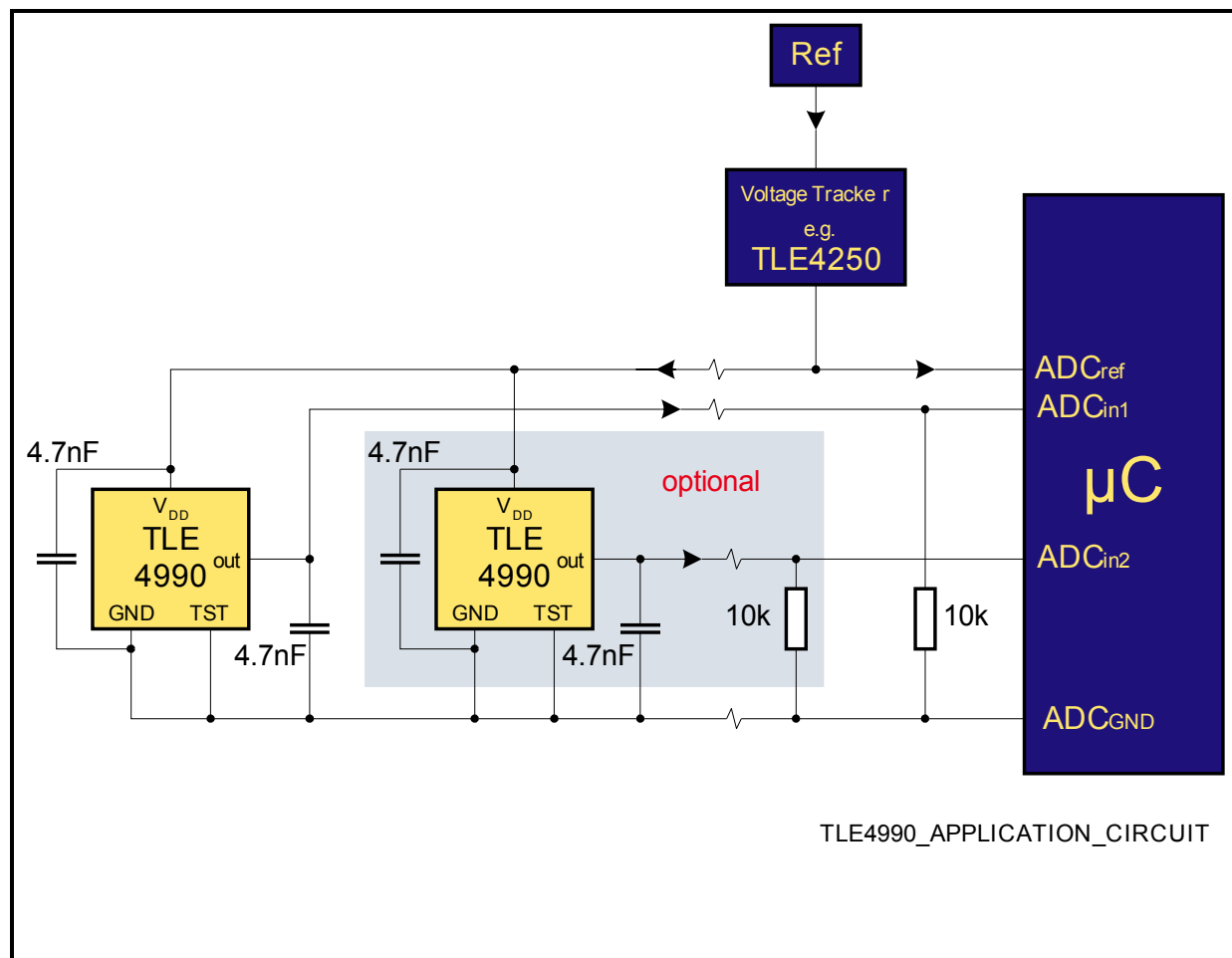
Figure 6 Application Circuit
