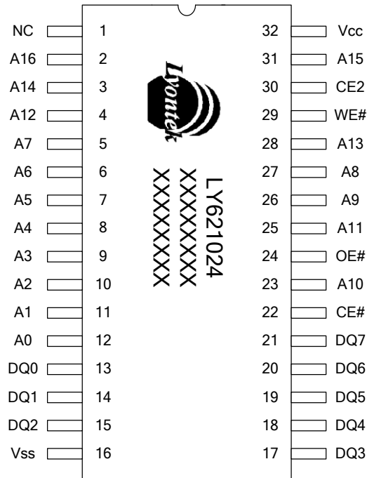
SOP/PDIP
