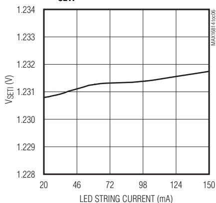
VSETI vs. PROGRAMMED CURRENT
