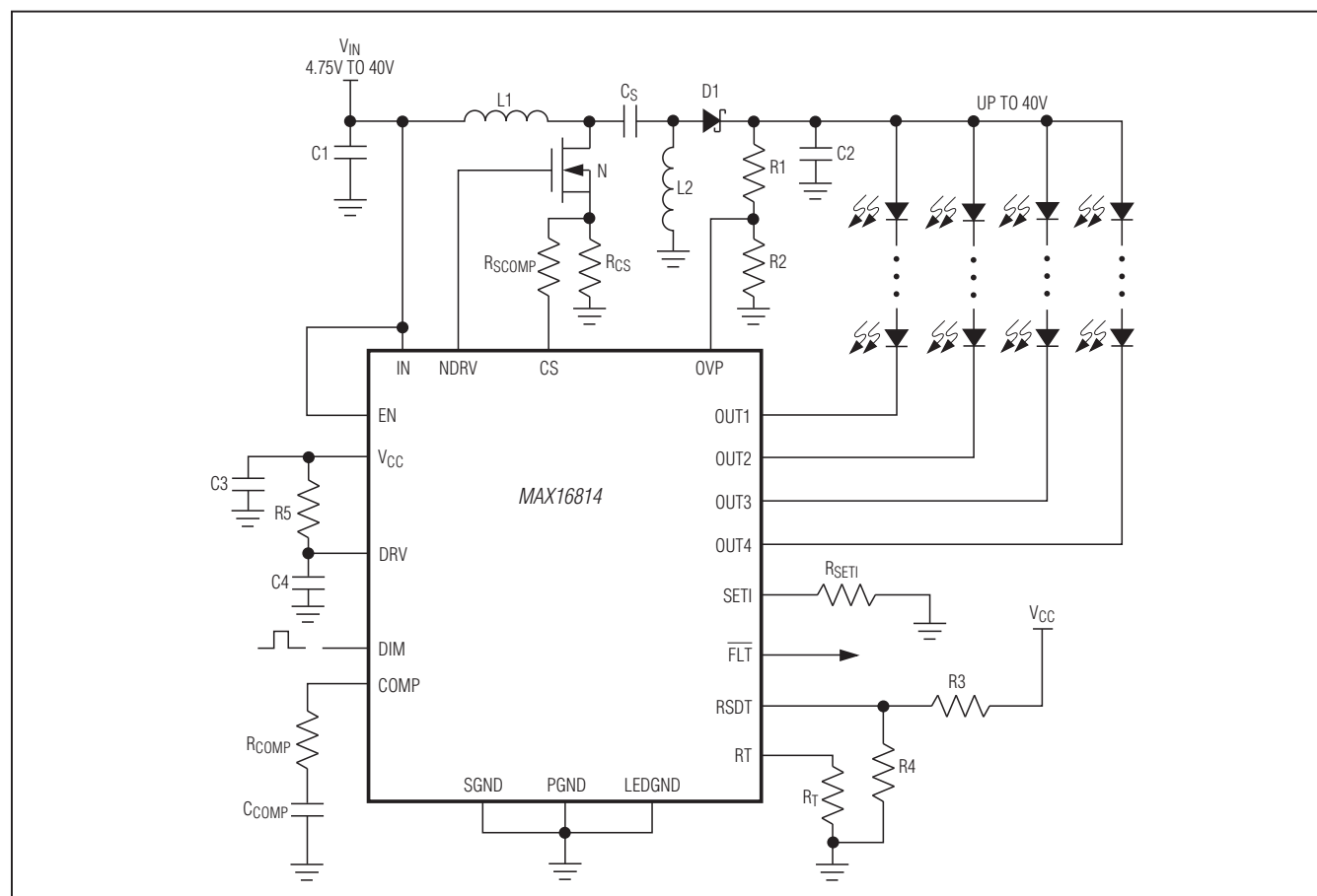
Figure 5. SEPIC Configuration
